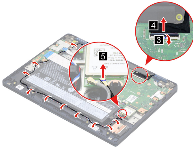
Figure 17. Disconnect EDP cable and antenna cable
