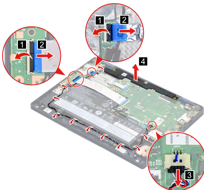
Figure 6. Remove the speaker
