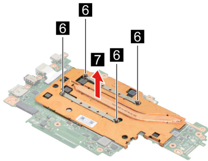
Figure 15. Remove the heat sink
