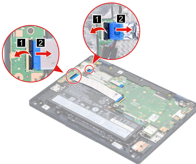
Figure 9. Disconnect cables connected to the I/O board
