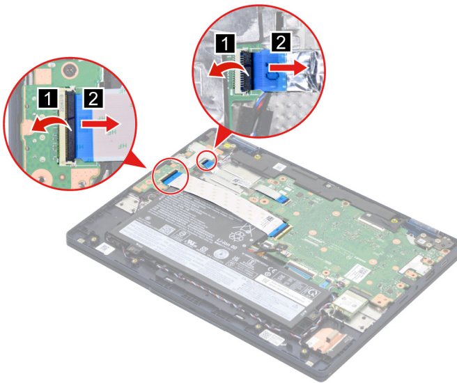
Figure 16. Disconnect the I/O board cable from the I/O board
