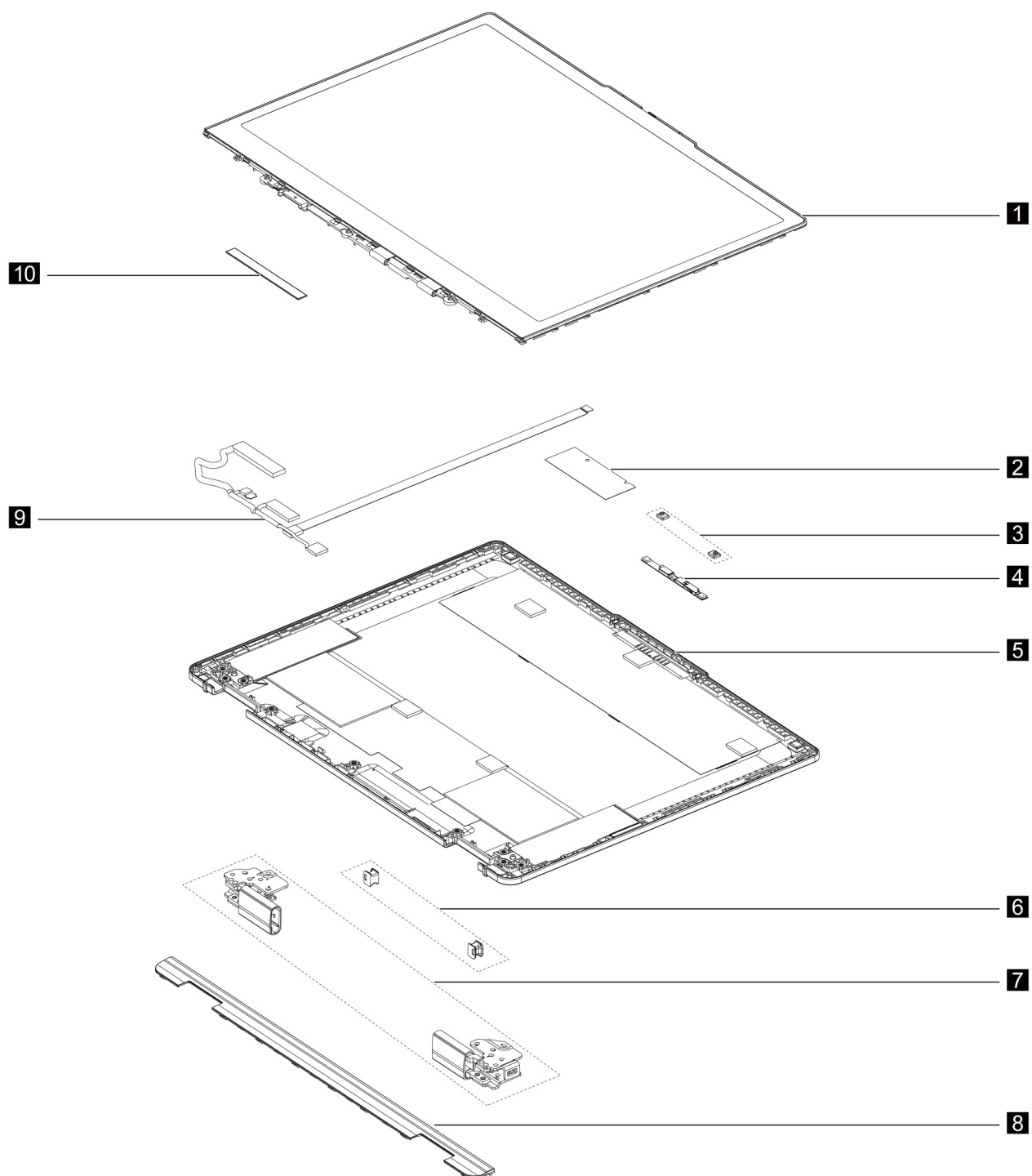
Figure 2. LCD module - exploded view
