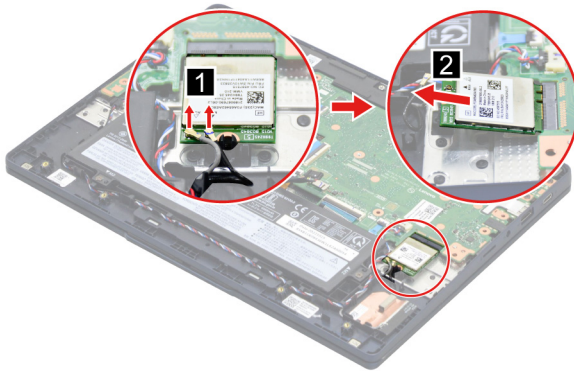
Figure 7. Remove the Wi-Fi card
