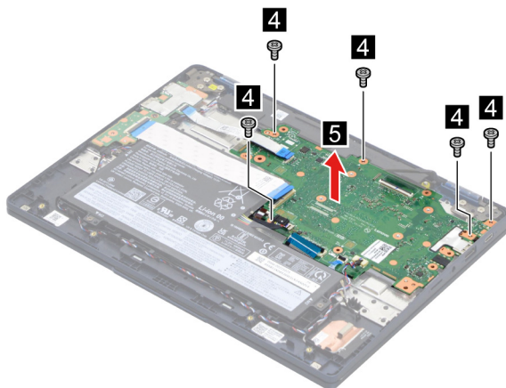
Figure 14. Remove five screws and remove the system board
