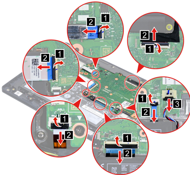
Figure 13. Disconnect cables connected to the system board
