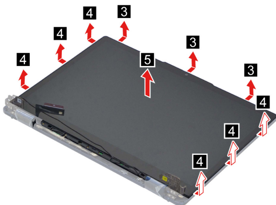
Figure 22. Remove the LCD panel
