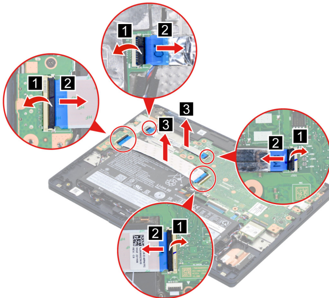
Figure 8. Remove the I/O board cable
