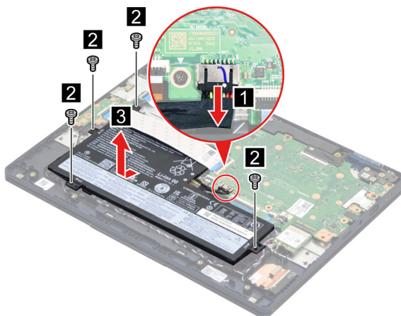
Figure 5. Remove the battery pack
