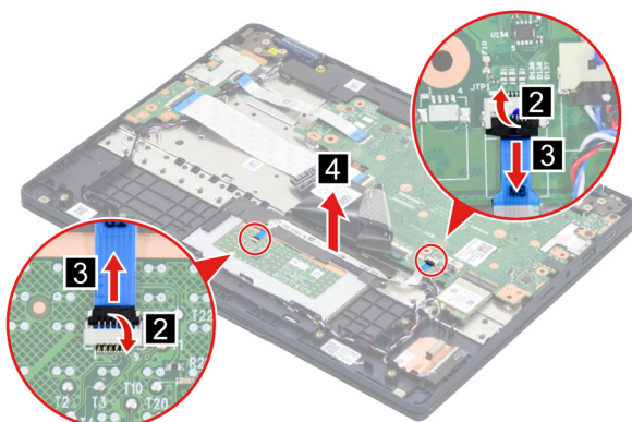
Figure 12. Remove the touchpad board cable
