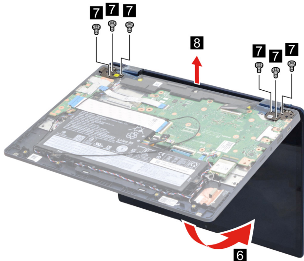
Figure 18. Remove the LCD module
