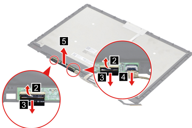
Figure 24. Remove the sensor board
