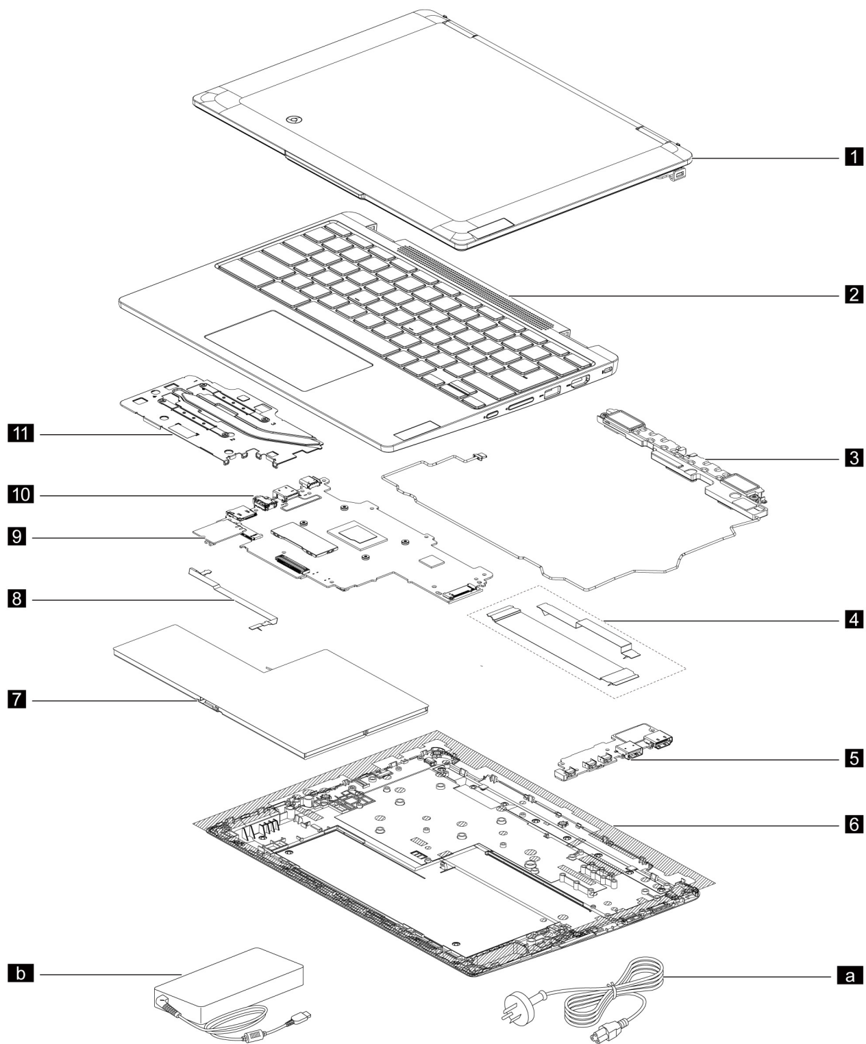
Figure 1. exploded view
