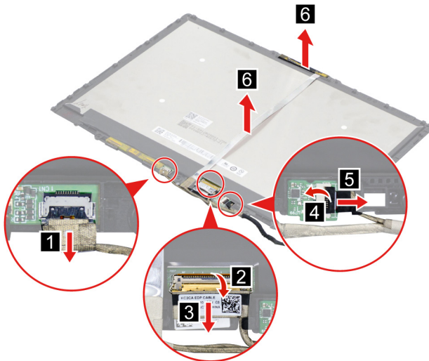
Figure 26. Remove the camera board and the EDP cable
