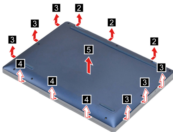
Figure 4. Pry up the latches and remove the lower case
