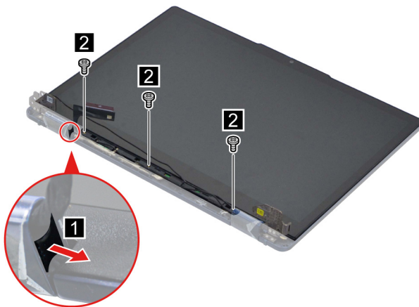
Figure 21. Remove the hinge rubber and remove three screws
