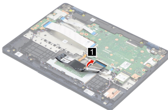
Figure 11. Peel back the keyboard cable
