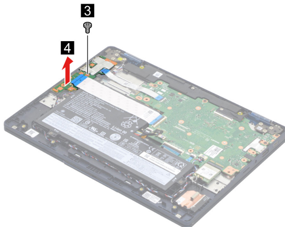
Figure 10. Remove one screw and remove the I/O board
