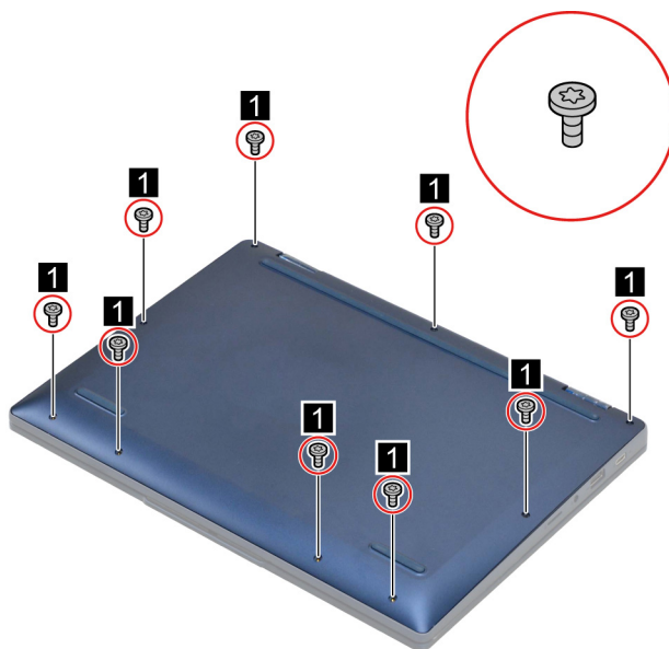
Figure 3. Remove nine screws
