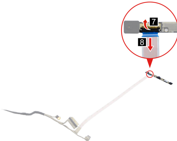
Figure 27. Separate the EDP cable from the camera board
