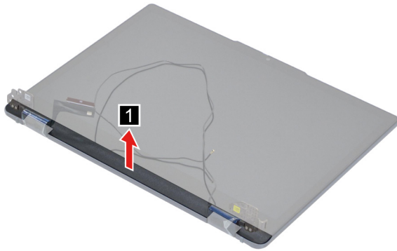
Figure 20. Remove the strip cover
