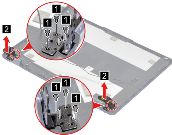
Figure 29. Remove six screws and remove the hinges
