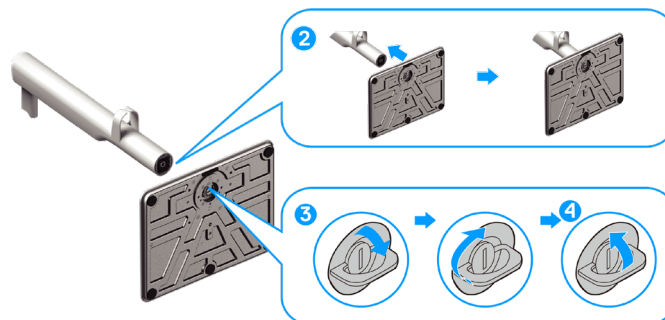
Figure 12. Install the stand riser and stand base
