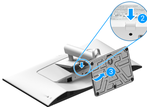
Figure 23. Removing the monitor stand
