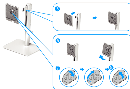
Figure 13. Install the VESA cover and stand riser
