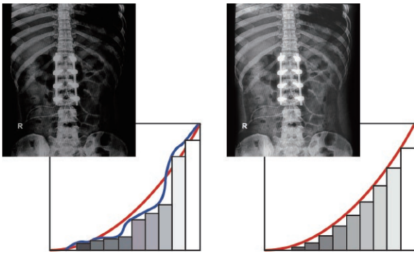
DICOM Mode
