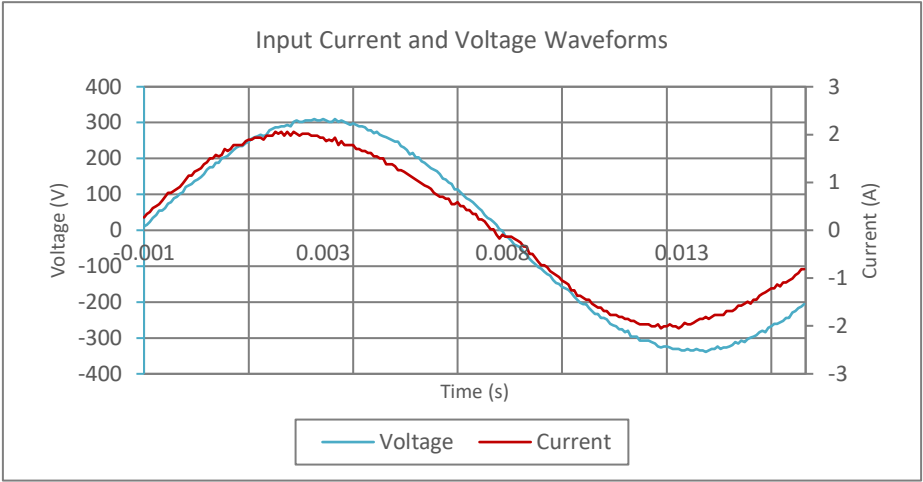
Input AC Current Waveform (ITHD = 6.35%, 50% Load)
