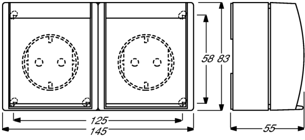
ocean® 2gang horizontal SCHUKO® socket outlets with drilling dimensions
