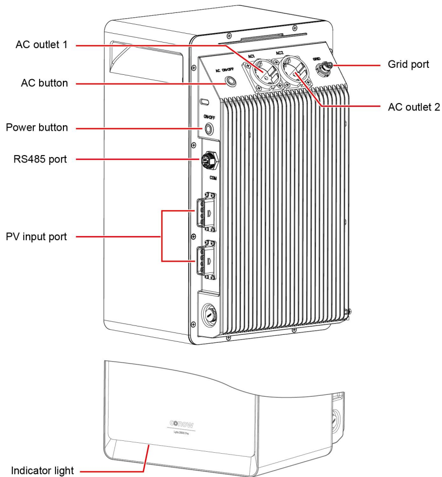
Figure 2-1 Lyra 2500 Pro
