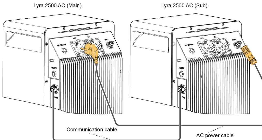
Figure 4-6 Installing the parallel cables
