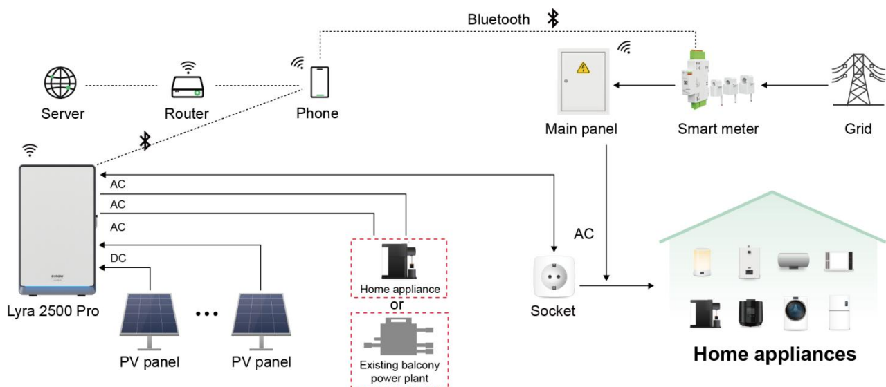
Figure 2-1 Network diagram
