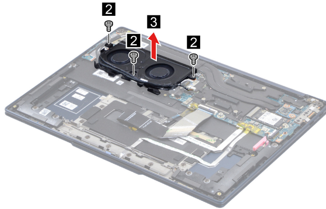
Figure 9. Remove three screws and remove the fan
