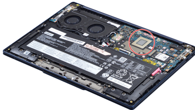
Figure 12. Areas on the system board where thermal interface materials are applied
