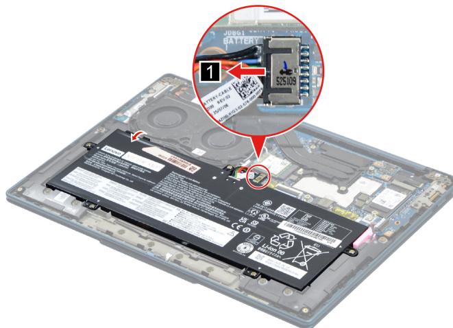
Figure 5. Disconnect the battery cable
