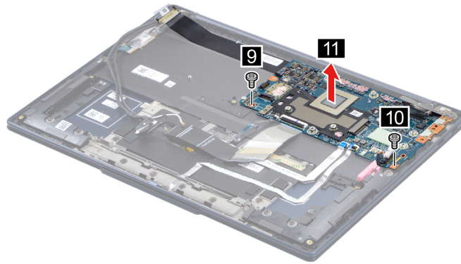
Figure 19. Remove two screws and remove the system board
