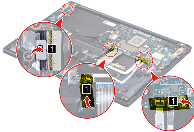
Figure 17. Remove the adhesive tape
