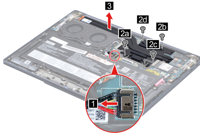
Figure 10. Remove four screws and remove the heat sink
