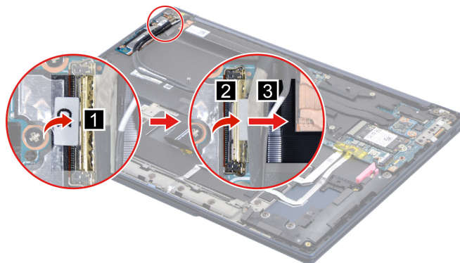
Figure 21. Disconnect the IO board cable
