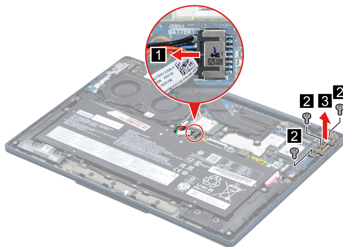
Figure 16. Remove three screws and remove the USB-C bracket
