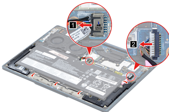
Figure 23. Disconnect the speaker cable
