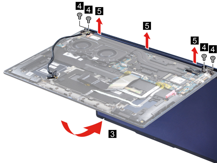
Figure 31. Rotate the display module, remove four screws and remove the display module
