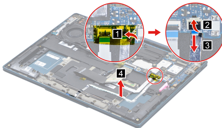
Figure 25. Remove the microphone board with FFC
