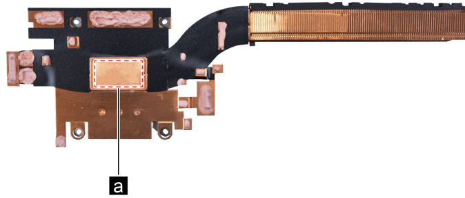
Figure 11. Areas on the heat sink where thermal interface materials should be applied
