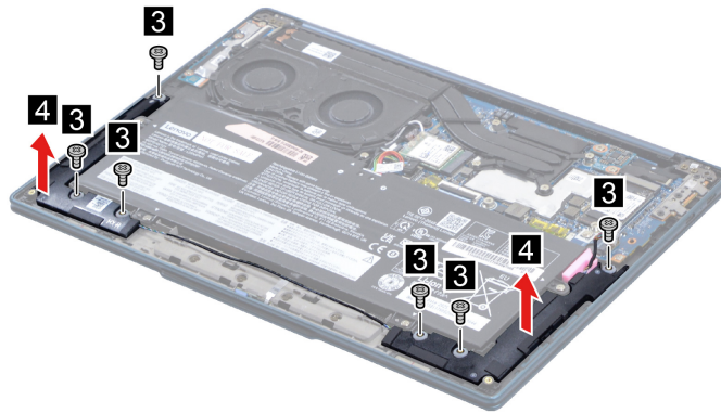
Figure 24. Remove six screws and remove the speakers
