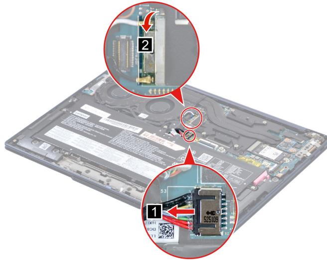
Figure 13. Remove the Wi-Fi card mylar
