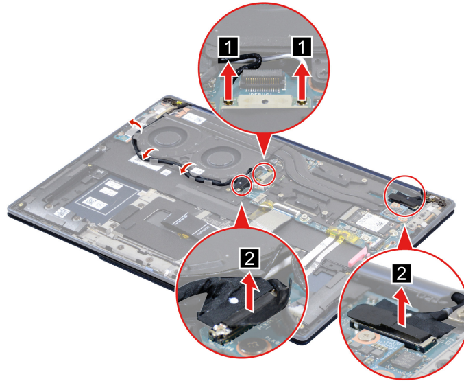
Figure 30. Disconnect the antenna cables, camera cable and EDP cable from the system board
