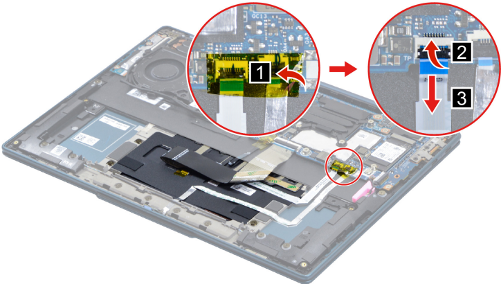
Figure 26. Remove the yellow adhesive tape and disconnect the touchpad FFC
