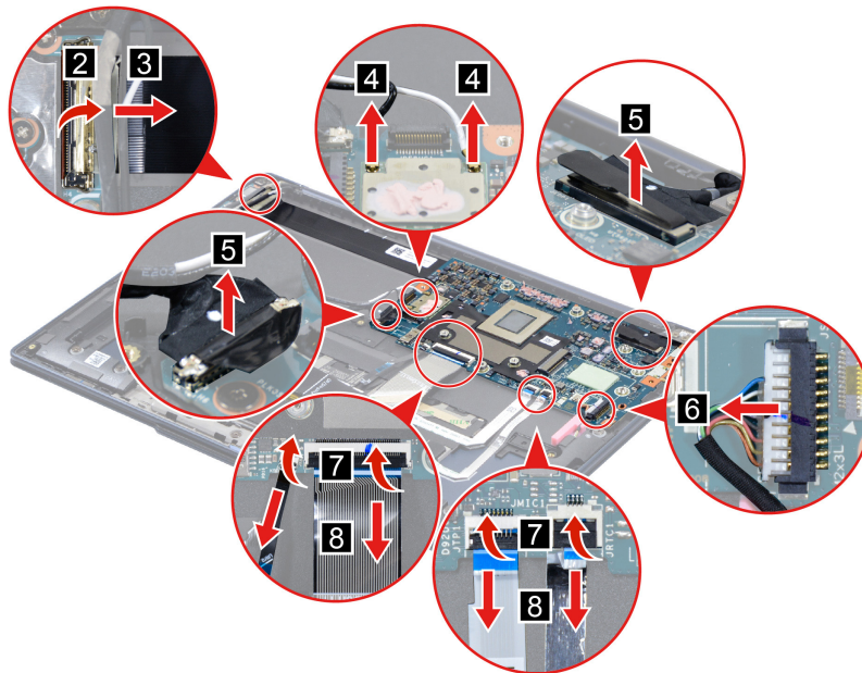
Figure 18. Disconnect cables
