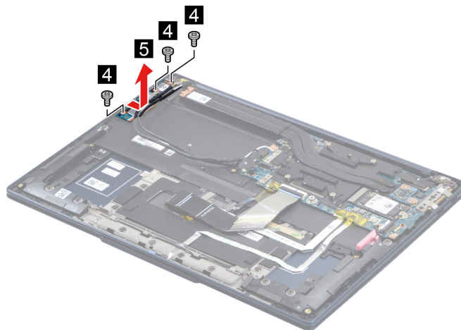
Figure 22. Remove three screws and remove the IO board
