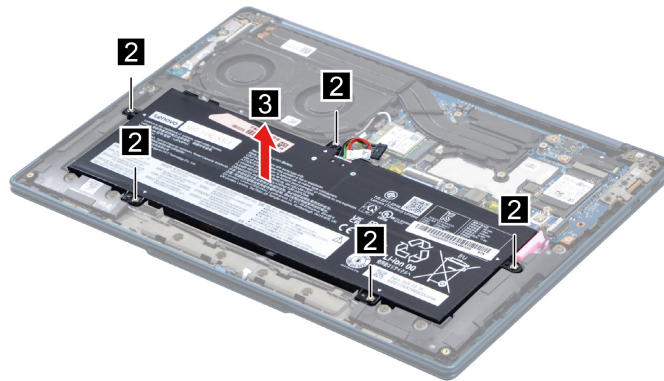
Figure 6. Remove five screws and remove the battery pack with cable
