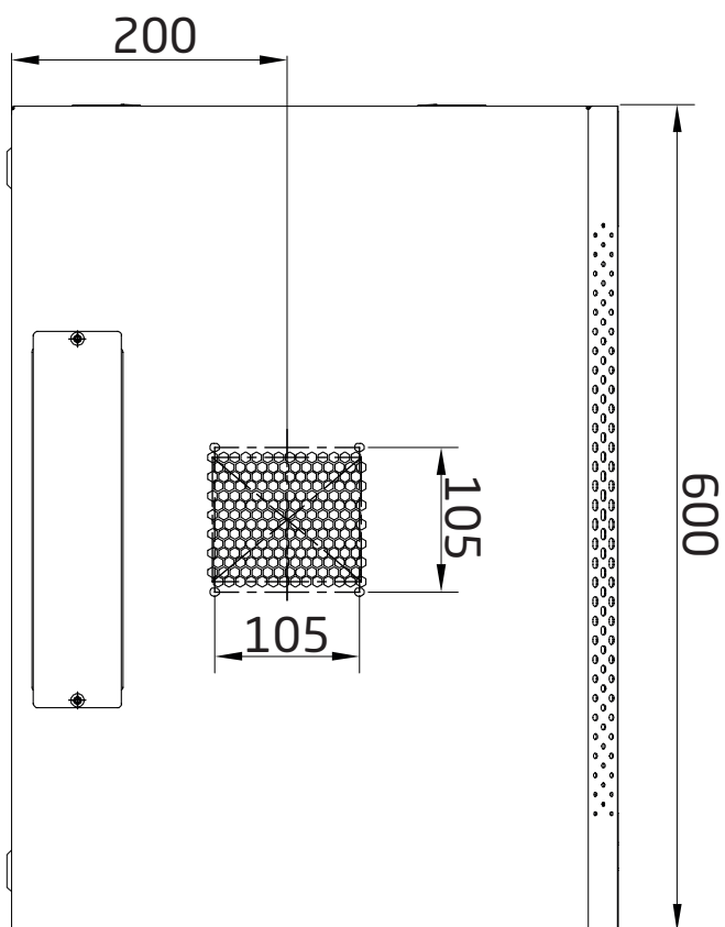
Deckel
