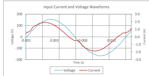
Input AC Current Waveform (ITHD = 8.88%, 50% Load)
