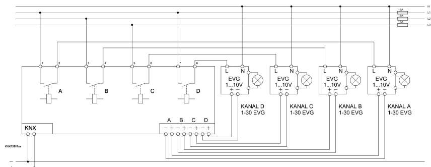
Exemplary circuit diagram AKD-0401V.02
