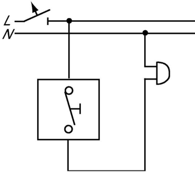
Push switch
