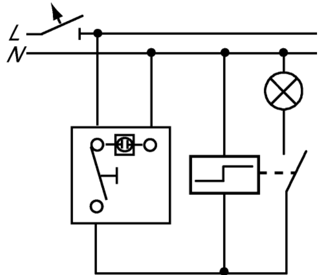
Push switch with relay (with neon indicator)
