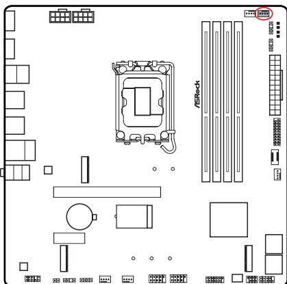
CPU_FAN2/WP
