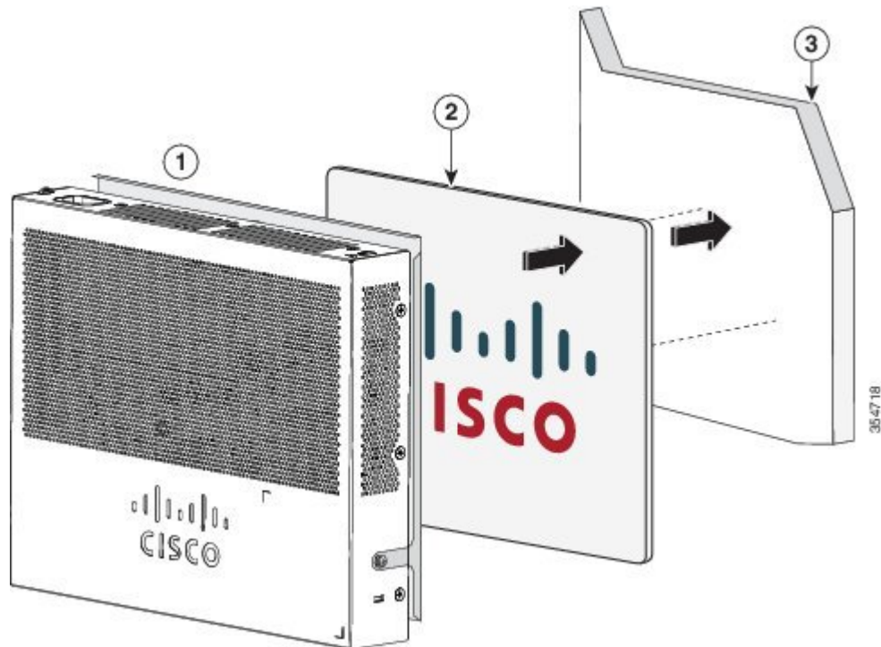
Figure 20: Wall-Mounting with a Magnet
