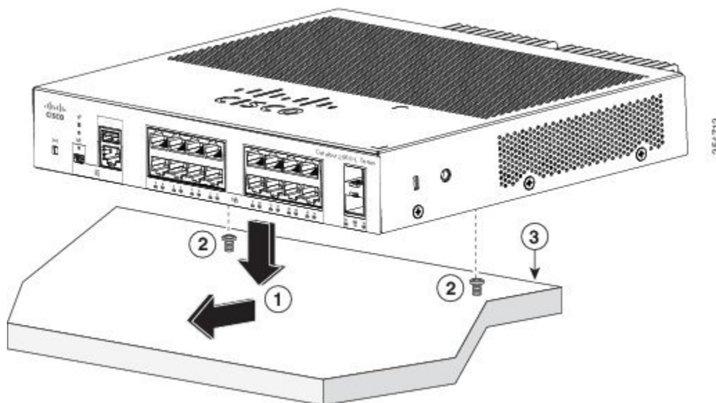
Figure 10: Mounting the Switch on Top of a Desk or Shelf
