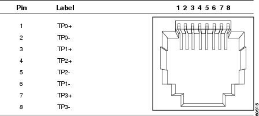
Figure 40: 10/100/1000 Port Pinouts
