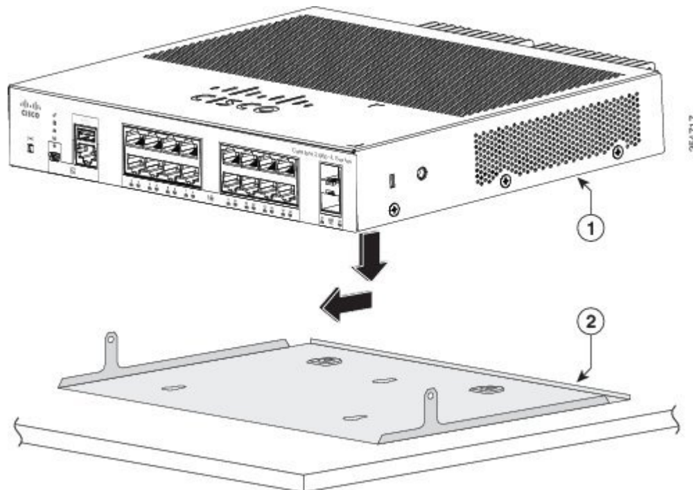
Figure 18: Placing the Switch on the Mounting Tray
