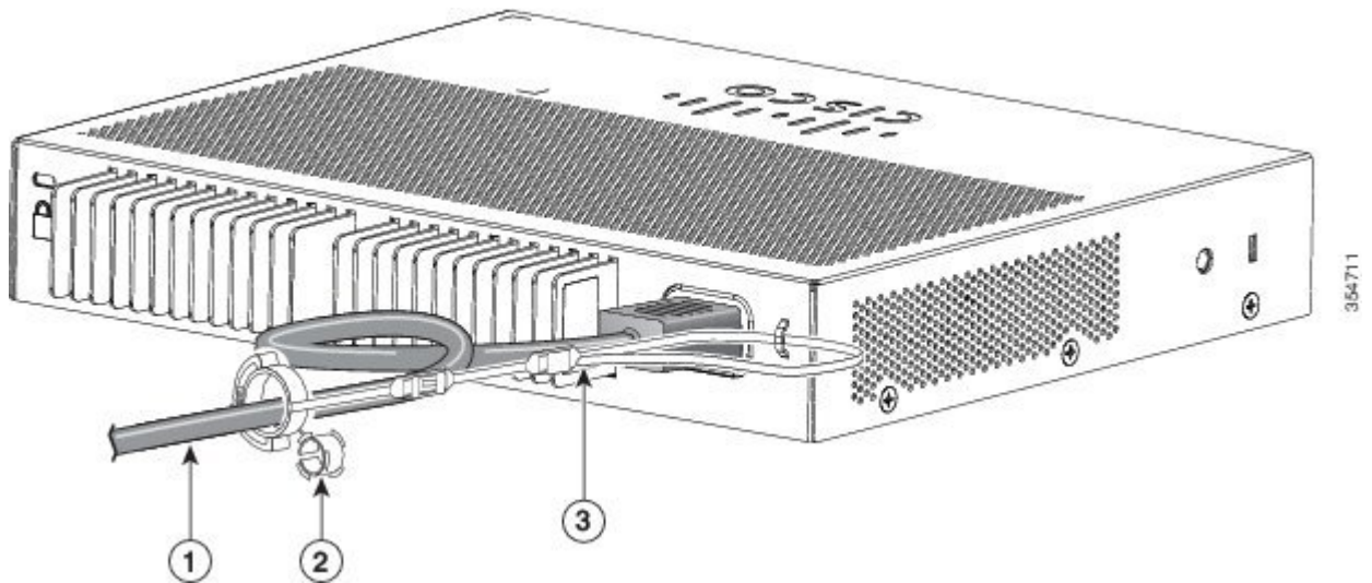
Figure 28: Sliding the Retainer Through the Latch
