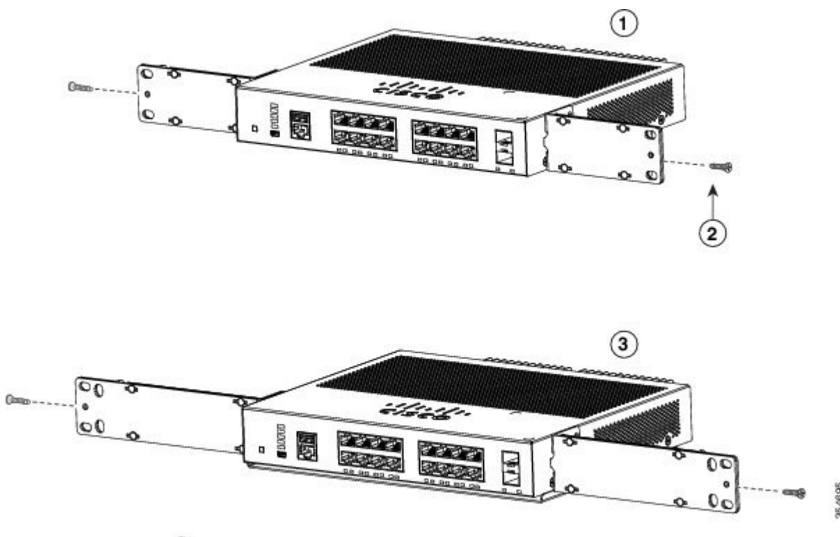
Figure 21: Attaching the 19-inch and 23-inch Brackets for Rack-Mounting
