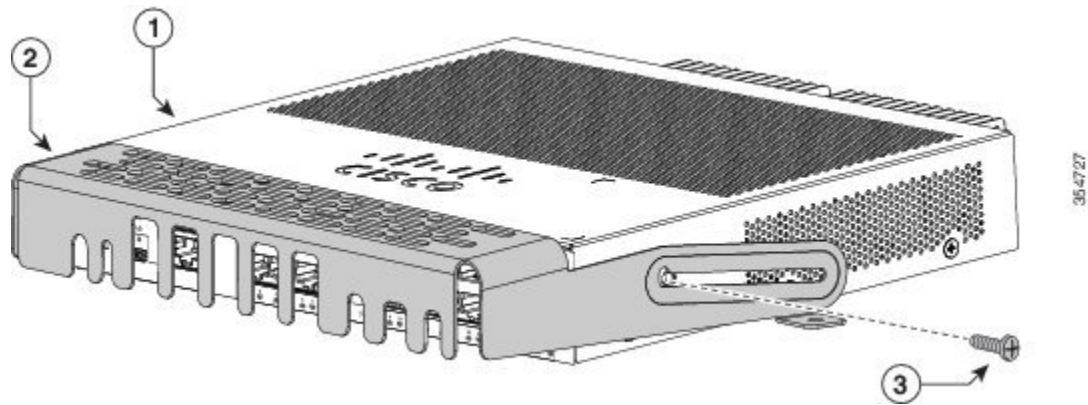
Figure 33: Attaching the Cable Guard to the Switch
