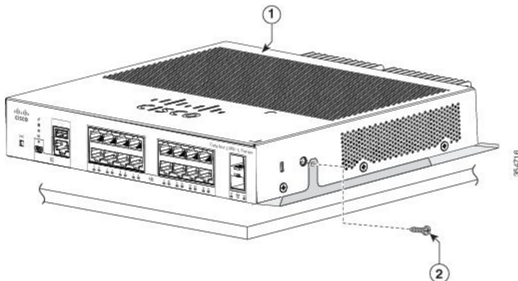
Figure 19: Securing the Mounting Tray to the Switch
