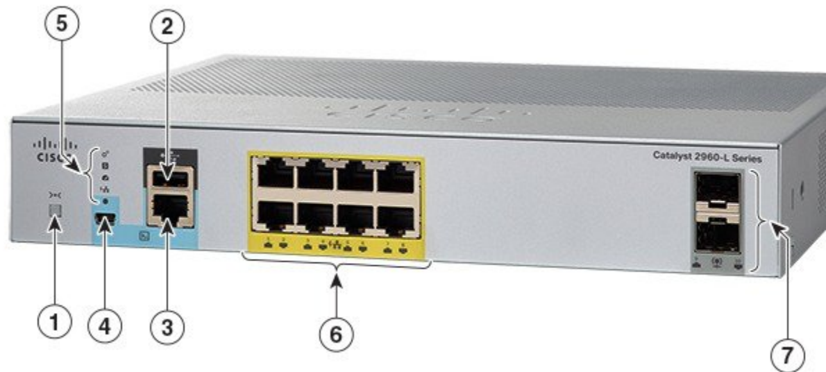
Figure 1: Front Panel of an 8-Port Cisco Catalyst 2960-L PoE Switch
