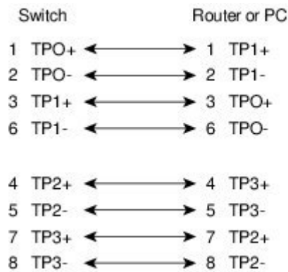
Figure 45: Four Twisted-Pair Semi-Cross Cable Schematic
