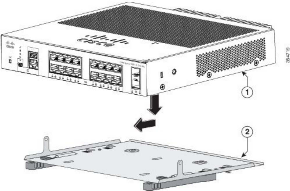
Figure 23: Placing the Switch on the DIN-Mount Tray
