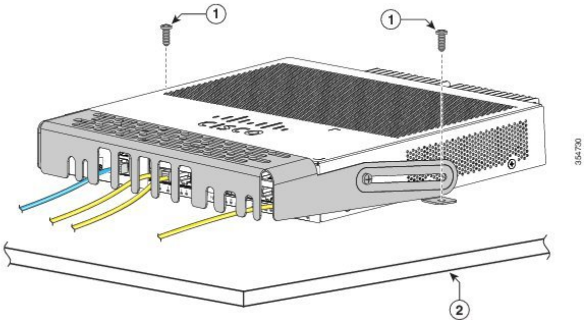
Figure 37: Securing the Cable Guard to the Desk
