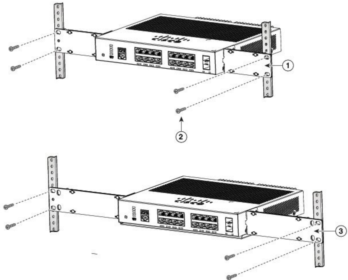
Figure 22: Mounting the Switch in a Rack
