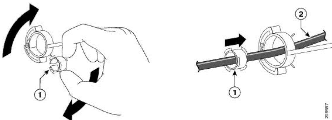
Figure 30: Sleeve Around the Power Cord
