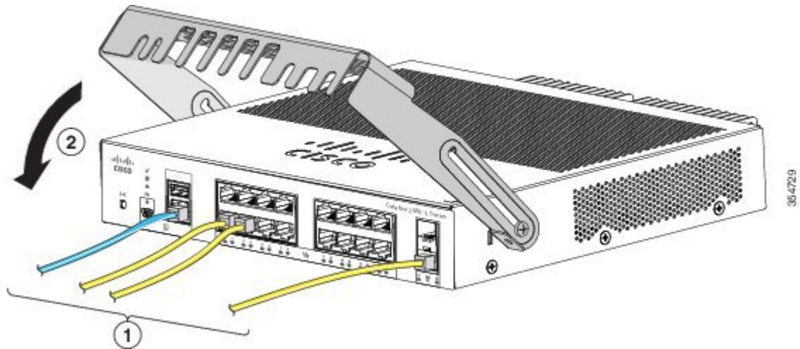
Figure 35: Attaching the Cables to the Switch
