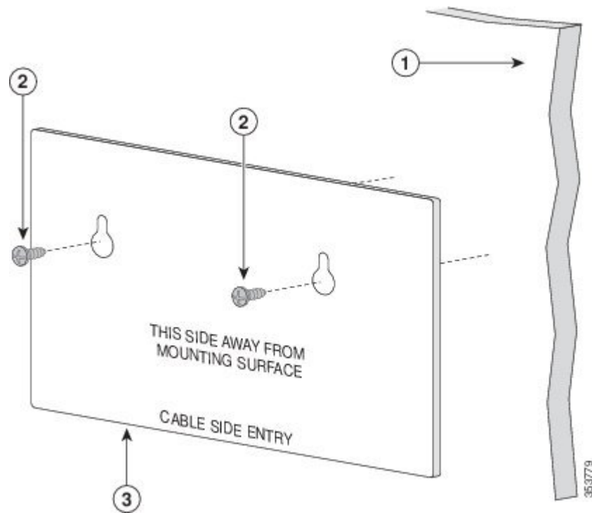
Figure 13: Installing the Mounting Screws on the Wall
