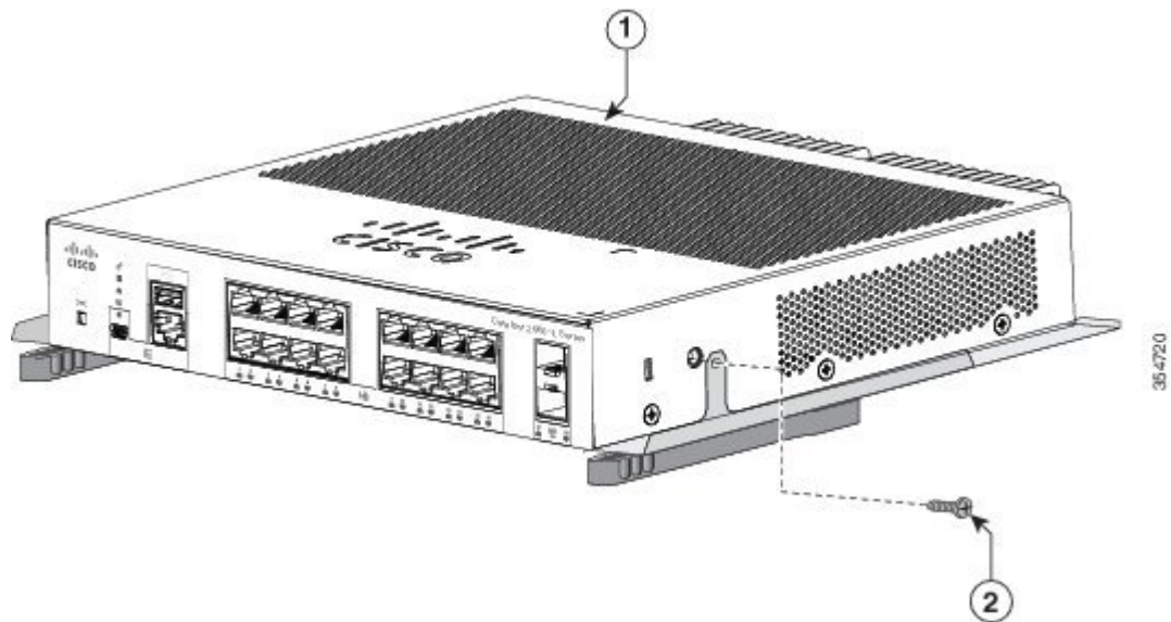
Figure 24: Securing the DIN-Mount Tray to the Switch
