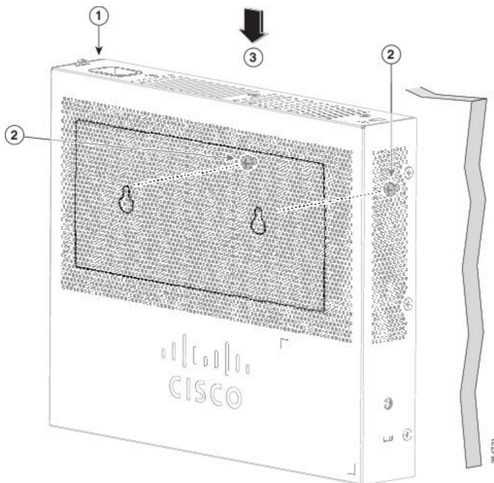
Figure 14: Installing the Switch on a Wall
