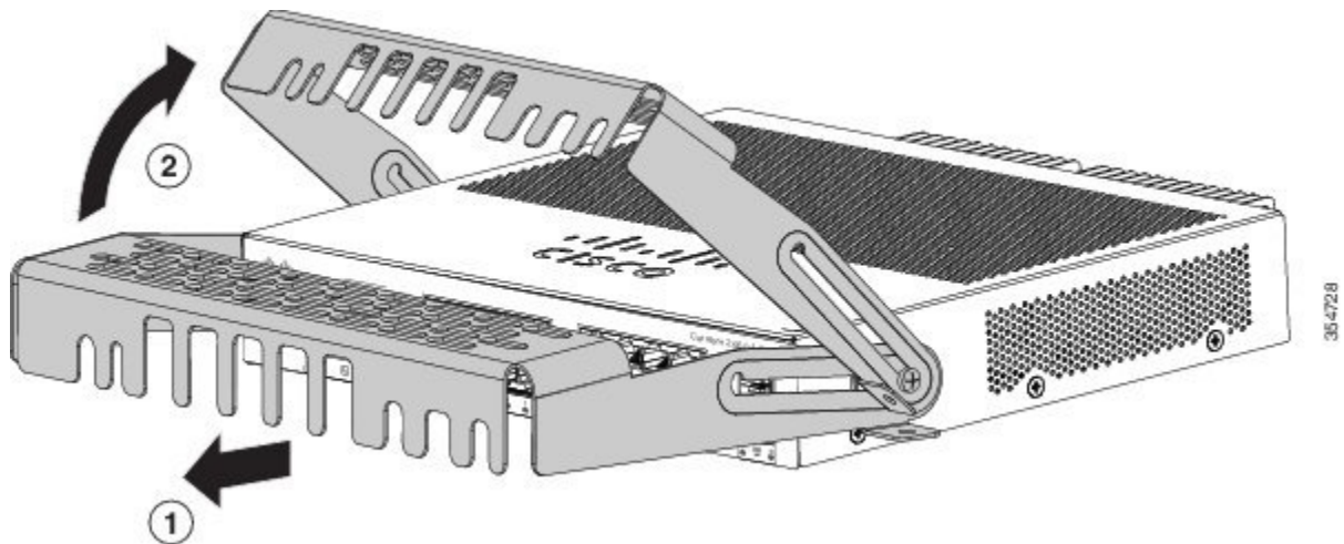
Figure 34: Pivoting the Cable Guard Upwards
