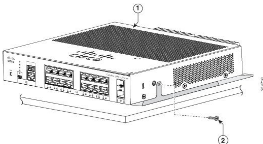
Figure 17: Securing the Switch to the Mounting Tray
