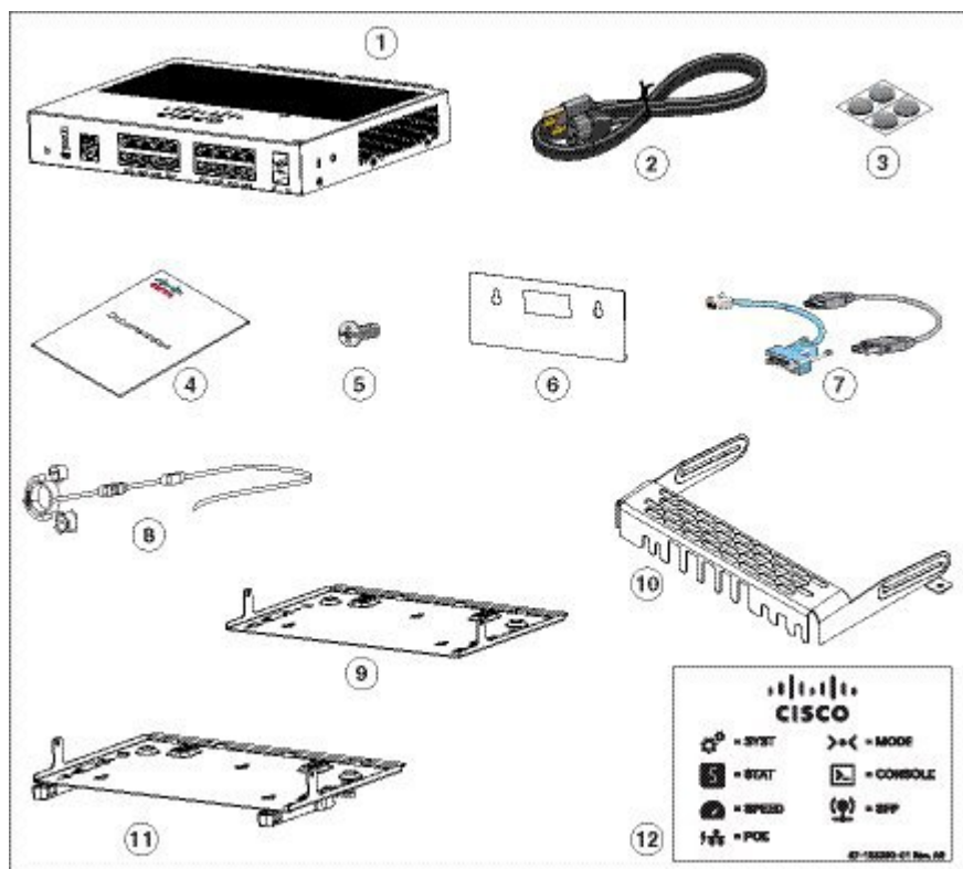
Figure 8: Box Contents of an 8-Port and 16-Port Cisco Catalyst 2960-L Switch
