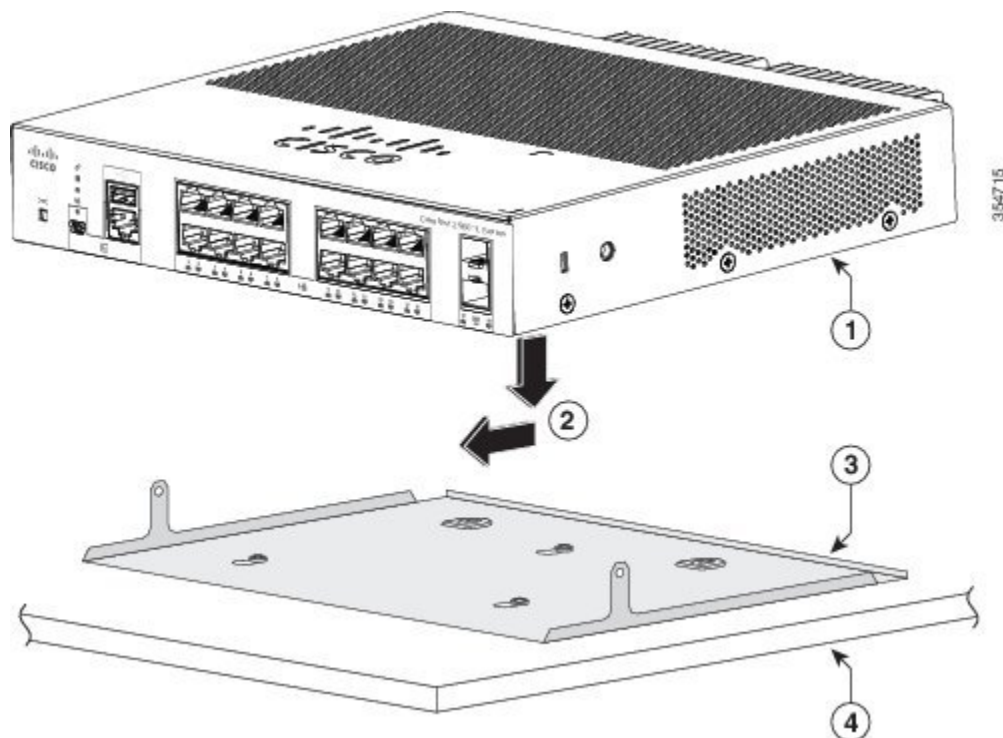
Figure 16: Installing the Switch on the Mounting Tray
