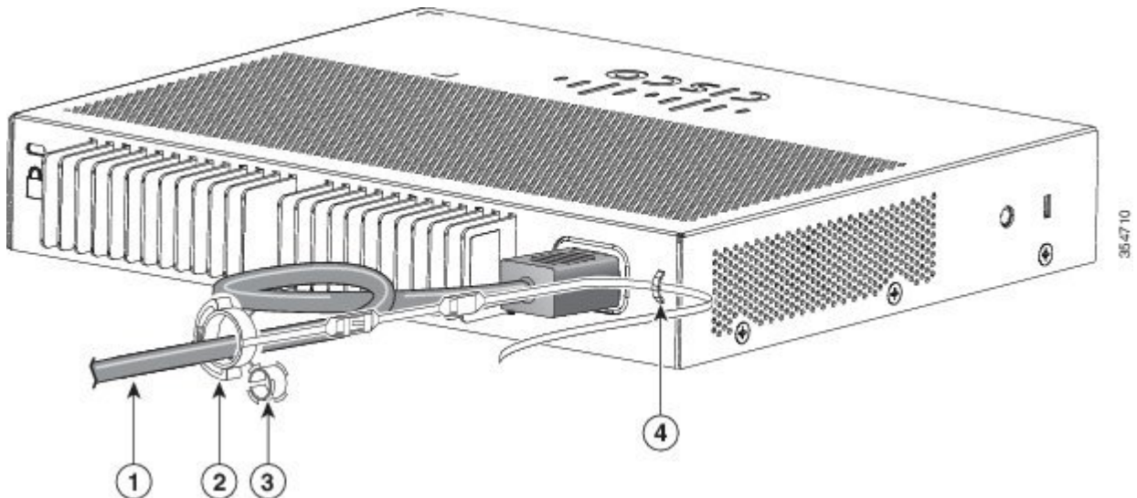
Figure 27: Inserting the Retainer through the Lanced Loop
