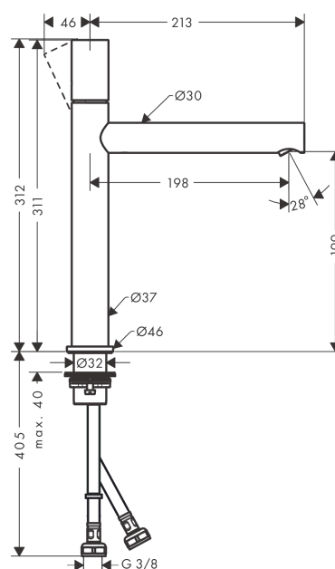
Scale drawing
