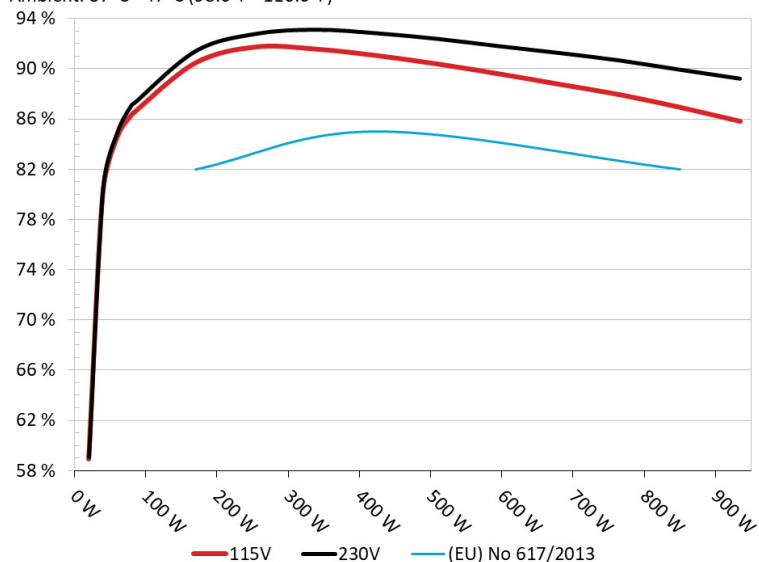
Efficiency: Thermaltake ToughPower GF2 ARGB 850W
