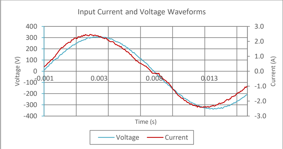
Input AC Current Waveform (ITHD = 7.73%, 50% Load)
