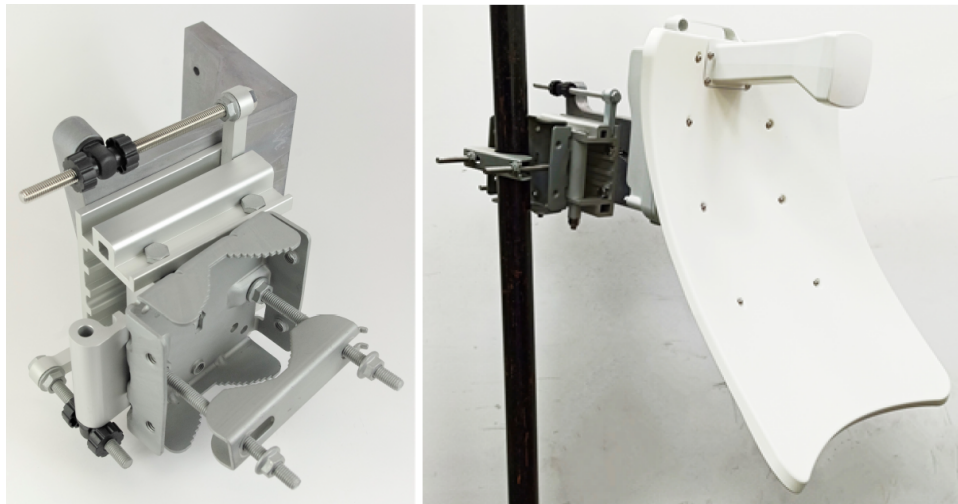
V3000 precision bracket components
