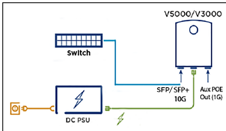
Figure 23: AC/DC powering diagram
