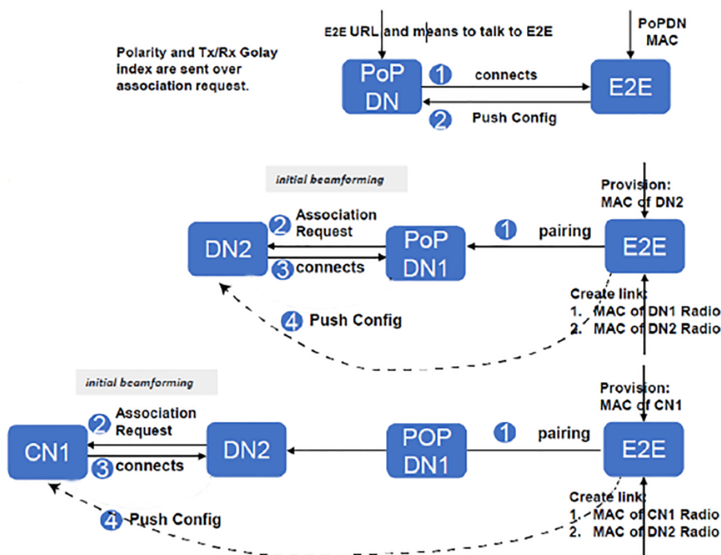
Figure 31: Nodes' deployment
