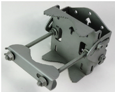
Figure 10 : Tilt bracket assembly
