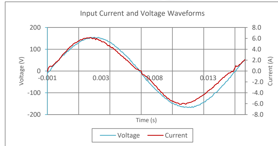
Input AC Current Waveform (ITHD = 6.98%, 50% Load)
