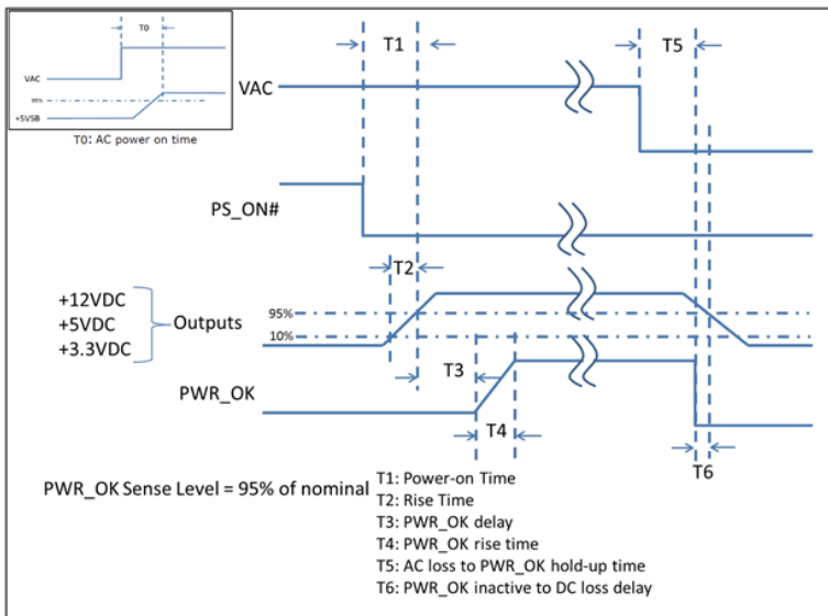
Figure 1 Time Diagram
