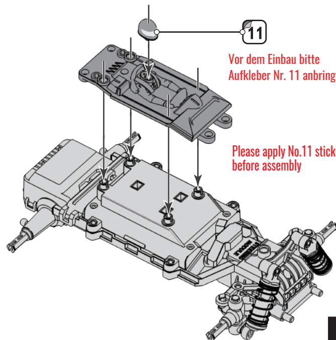
Helm / Helmet D1-2 1x
