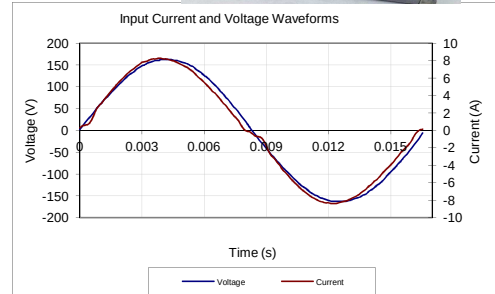
Input AC Current Waveform (ITHD = 6.2%, 50% Load)
