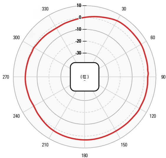
AZIMUTH 2.4 GHZ
