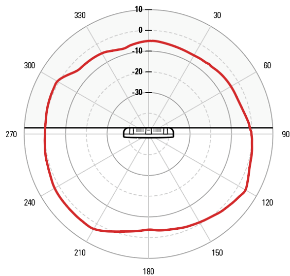
ELEVATION 5 GHZ
