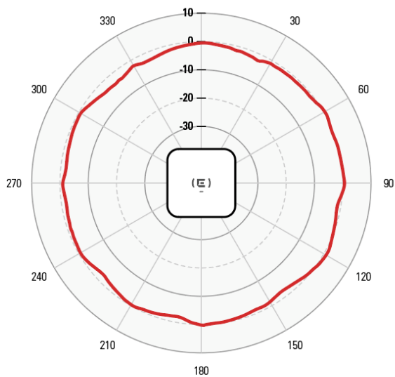
AZIMUTH 5 GHZ
