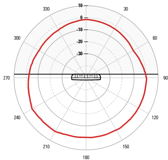
ELEVATION 2.4 GHZ
