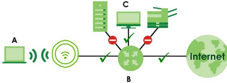
Figure 161 Layer-2 Isolation Application
