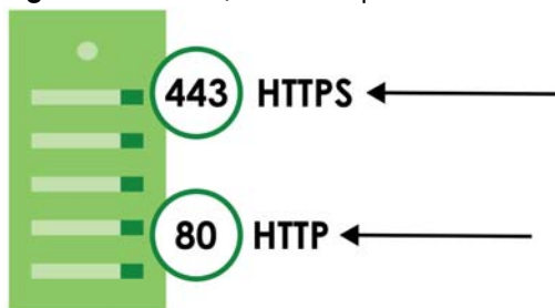
Figure 178 HTTP/HTTPS Implementation
