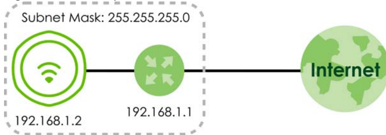
Figure 108 IP Setup
