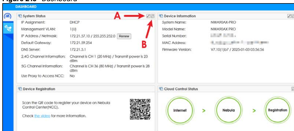
Figure 215 Dashboard
