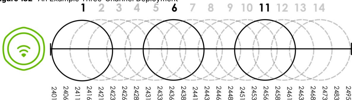
Figure 132 An Example Three-Channel Deployment
