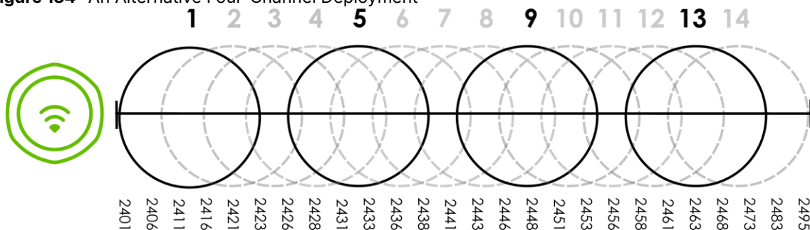
Figure 134 An Alternative Four-Channel Deployment
