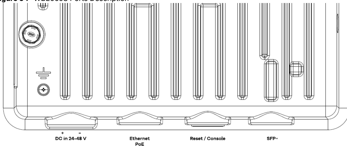
Figure 54 WBE665S Ports Description
