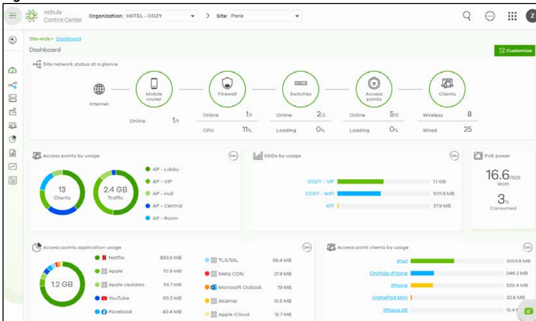
Figure 14 NCC Dashboard
