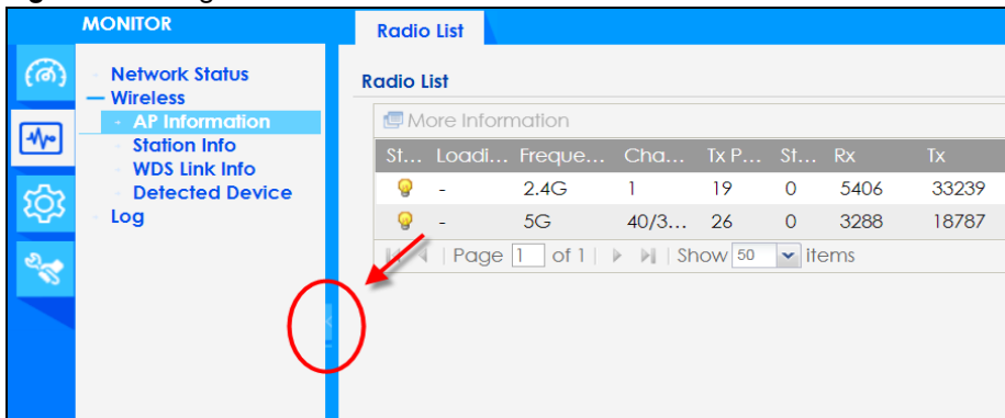
Figure 74 Navigation Panel
