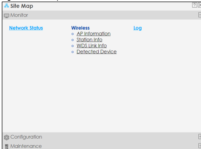
Figure 72 Site Map
