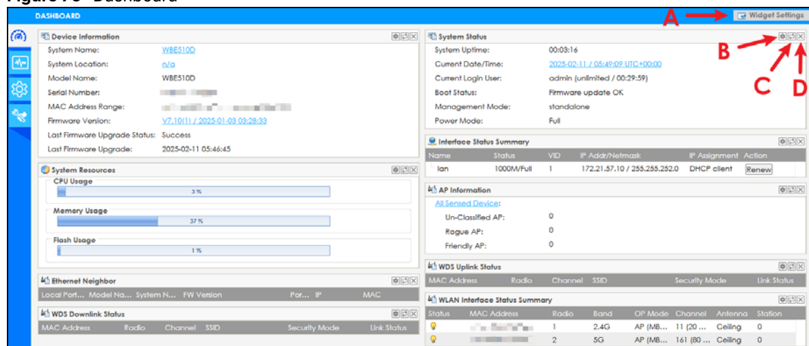
Figure 76 Dashboard
