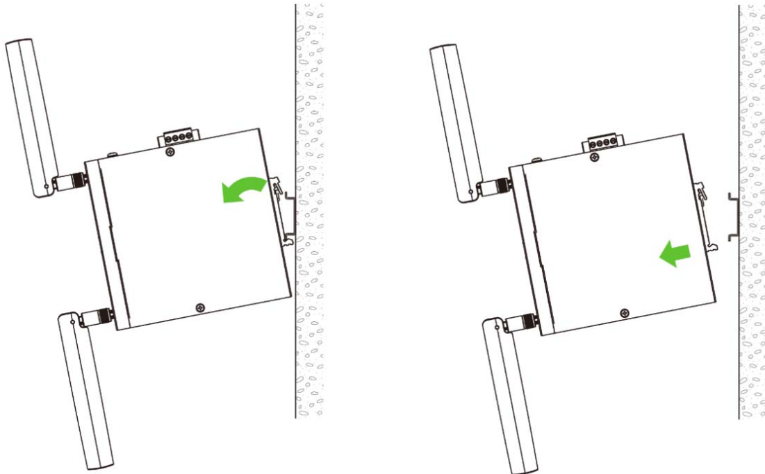
Figure 67 Remove the Zyxel Device
