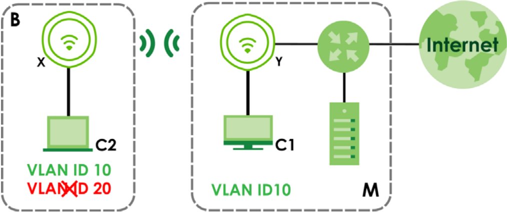
Figure 112 Wireless Bridge VLAN ID Example
