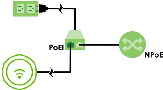
Figure 64 PoE Example Application - PoE Injector
