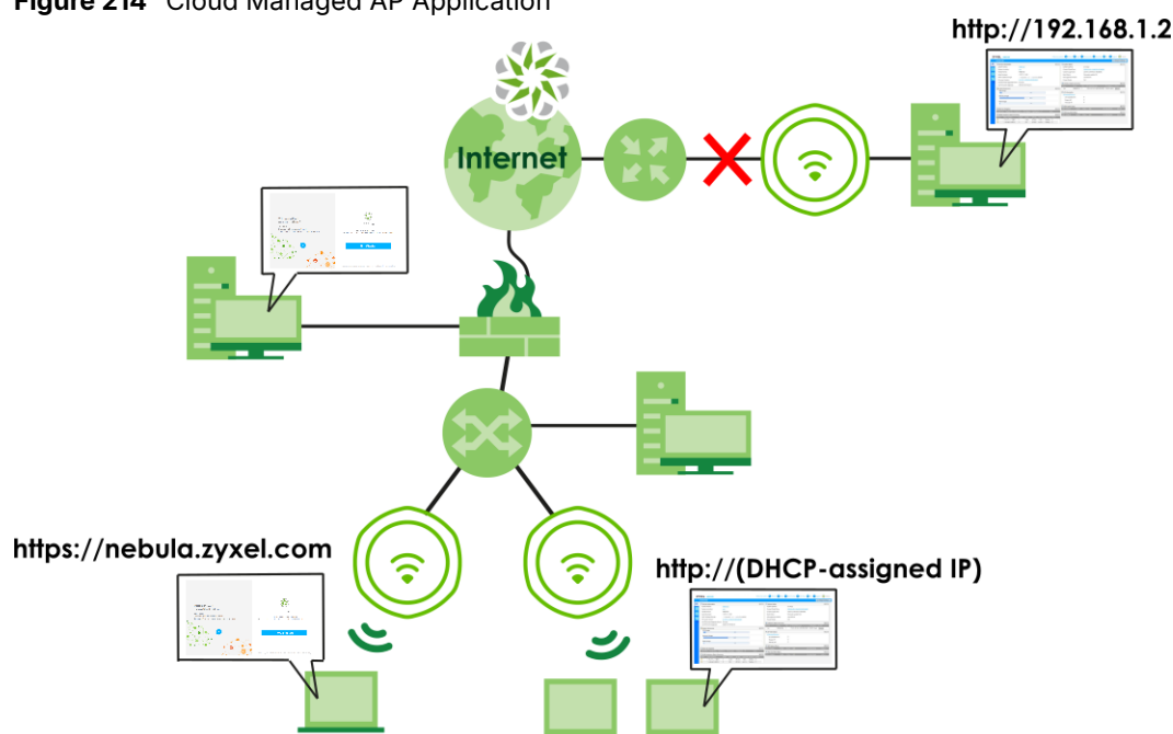
Figure 214 Cloud Managed AP Application
