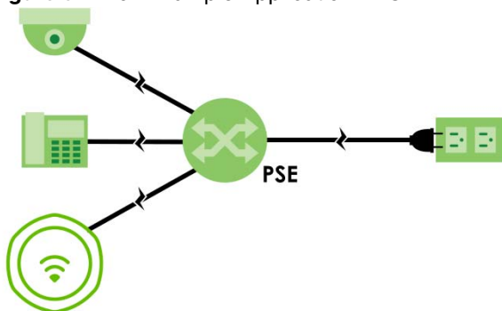
Figure 62 PoE Example Application - PSE
