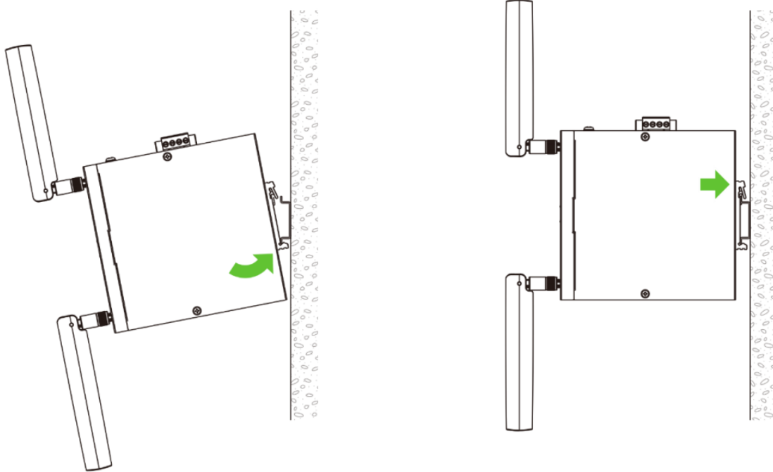
Figure 66 Attach the Zyxel Device
