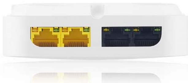
Figure 47 WAX300H Ports
