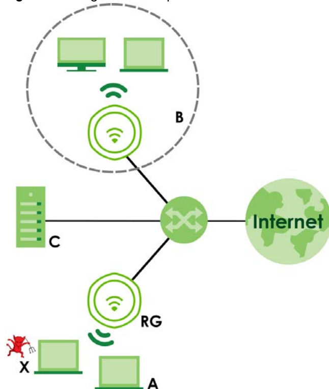
Figure 124 Rogue AP Example
