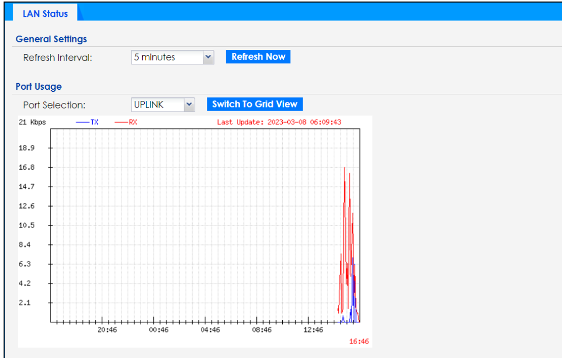
Figure 101 Monitor > Network Status > Switch to Graphic View
