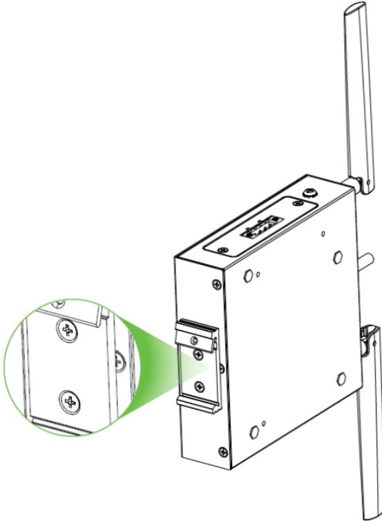
Figure 65 Attach the DIN-Rail bracket
