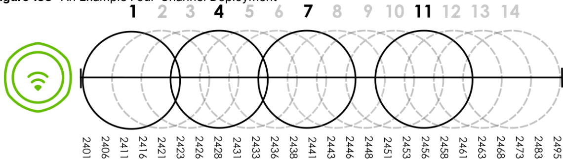
Figure 133 An Example Four-Channel Deployment
