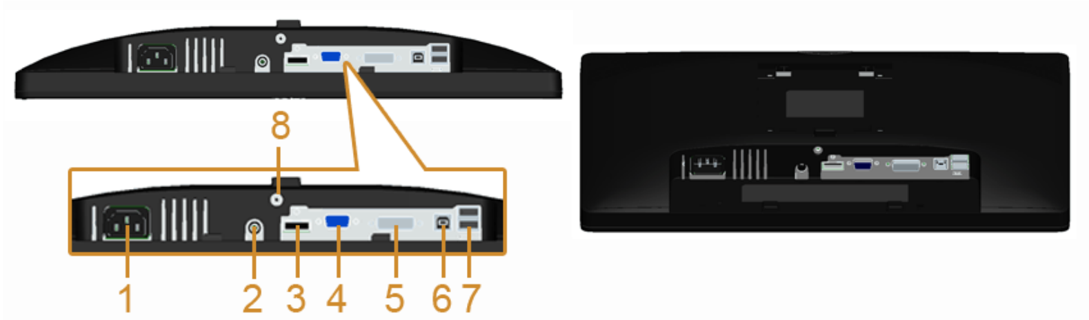
Bottom view without monitor stand
