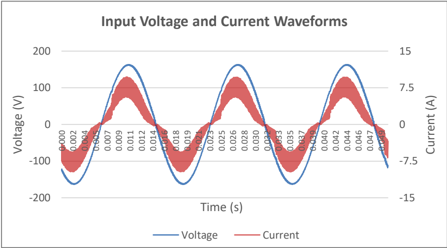
Input AC Current Waveform (ITHD = 14.42%, 50% Load)
