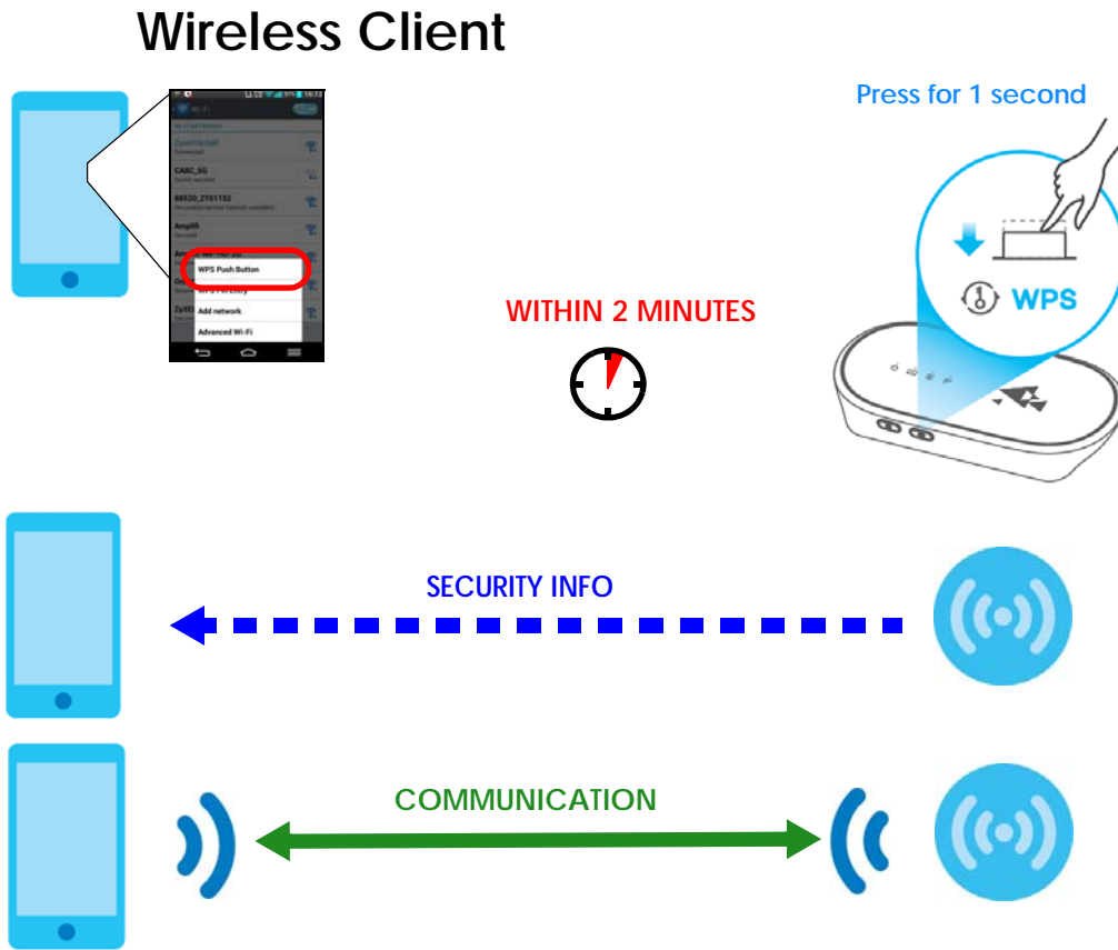
Figure 12 Example WPS Process: PBC Method
