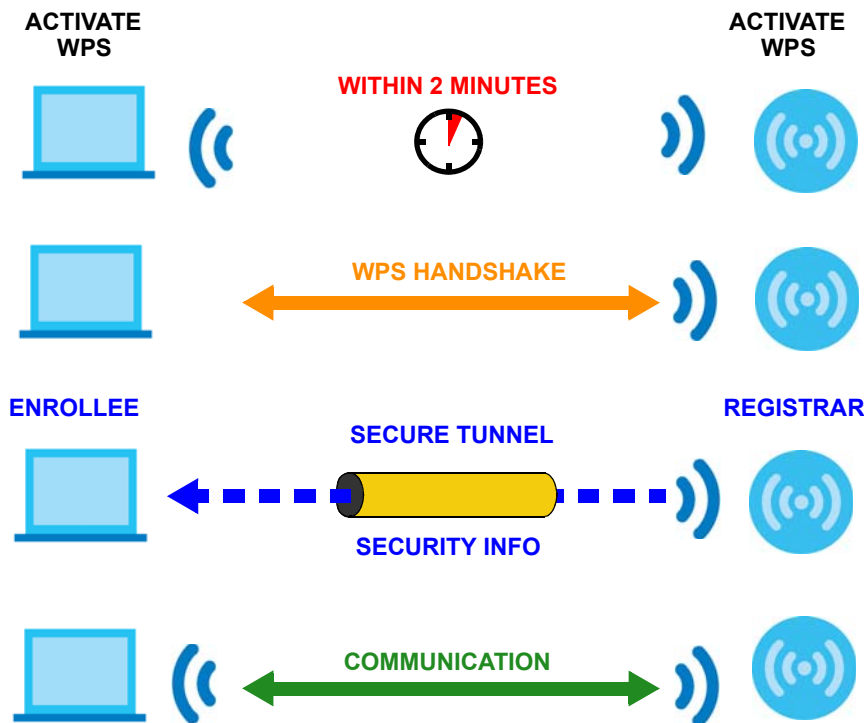
Figure 53 How WPS Works
