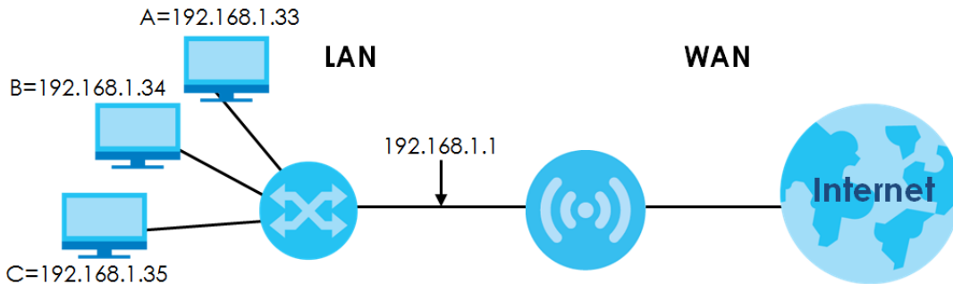
Figure 46 Multiple Servers Behind NAT Example
