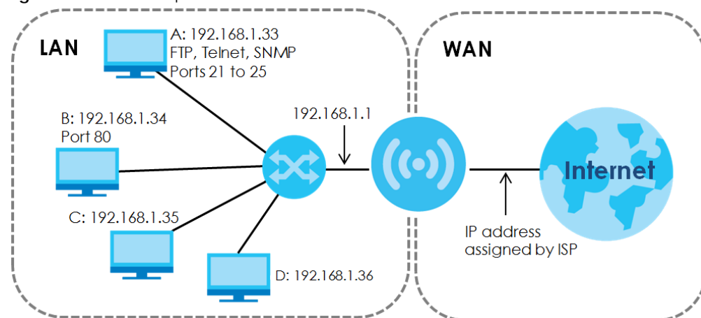
Figure 42 NAT Example
