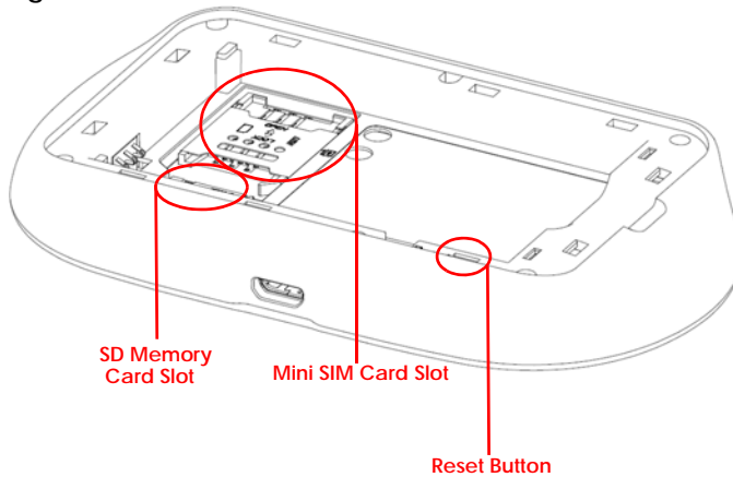
Figure 2 WAH7601 Interior Hardware
