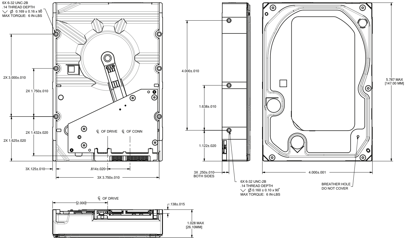
Figure 3. Mounting configuration dimensions 8TB models
