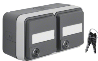
SCHUKO socket outlet 2gang horizontal with hinged cover surface-mounted with labelling field, Locks - differing lockings, enhanced contact protection, Berker W.1
