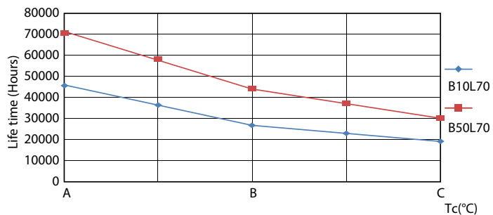
LEDtube_70K_LifetimeVsTc-LED
