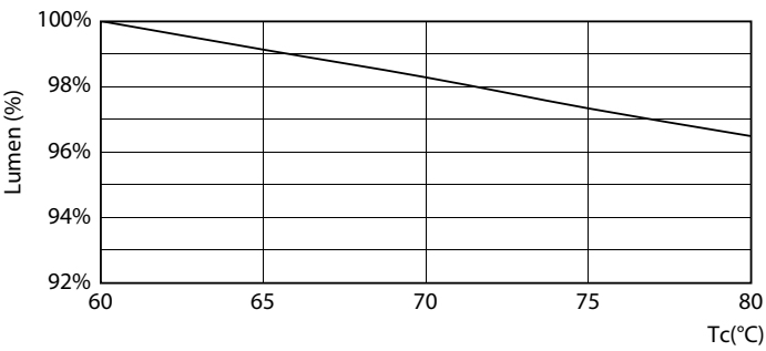
LEDtube MAS 21,7W 70K LumenVsTc
