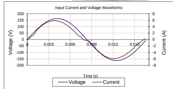
Input AC Current Waveform (ITHD = 9.78%, 50% Load)
