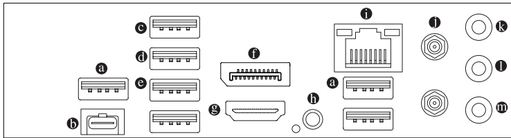
Back View-A
