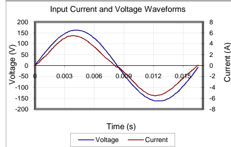
Input AC Current Waveform (ITHD = 8.99%, 50% Load)
