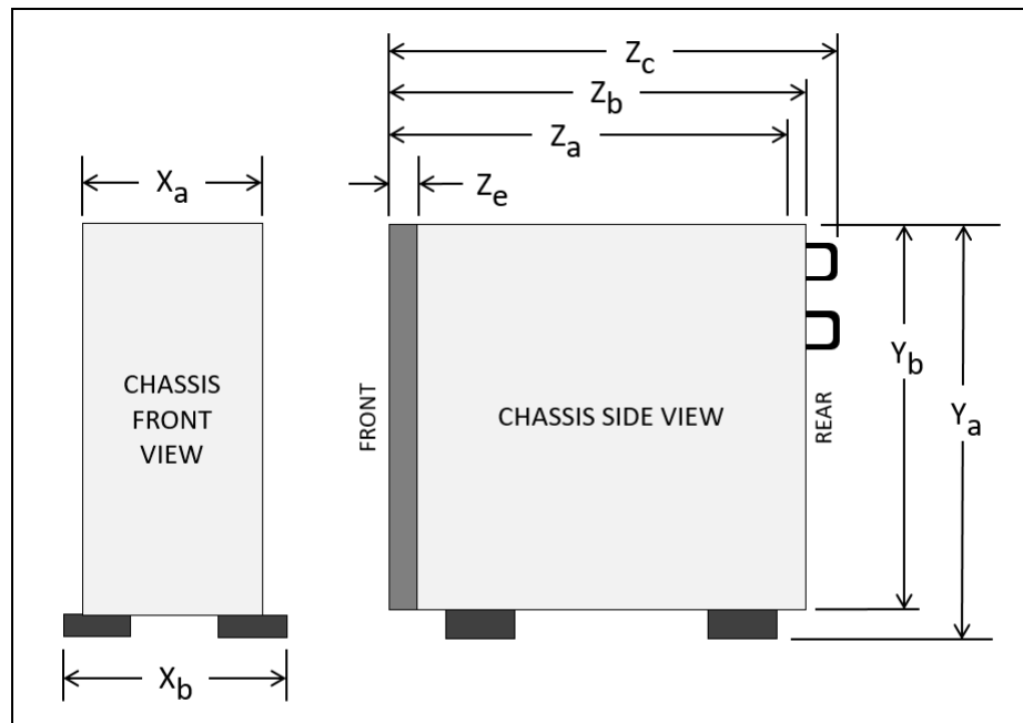
Figure 10. Server dimension
