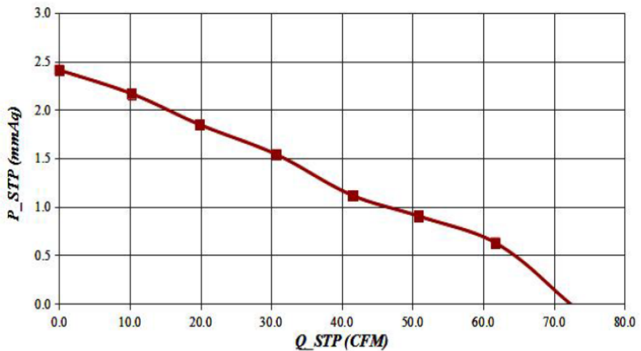
P-Q Curve
