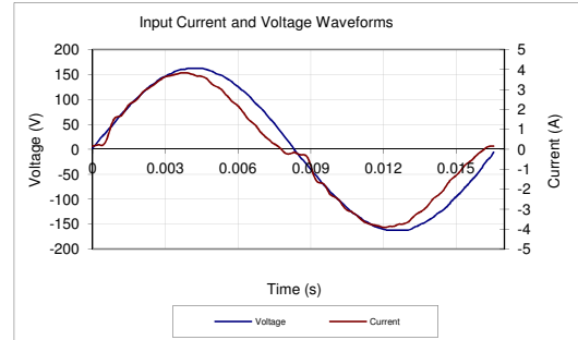
Input AC Current Waveform (ITHD = 12.01%, 50% Load)
