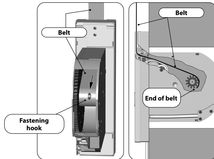
Belt path in RolloTron smart flush-mount- ed belt winder premium
