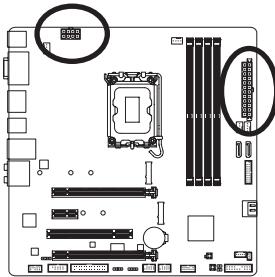
ATX_12V_2X4:
