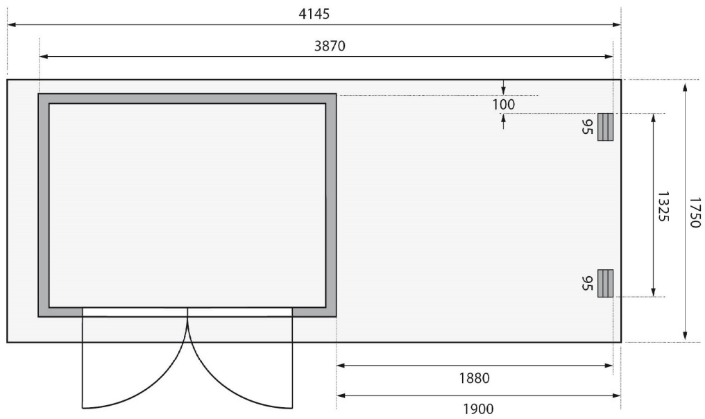
Fundamentplan (in mm)
