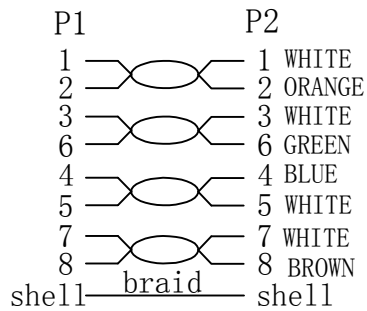
WIRING DIAGRAM(568B)
