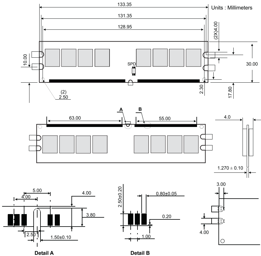
Figure 1: KVR533D2N4/2G 240-Pin DIMM
