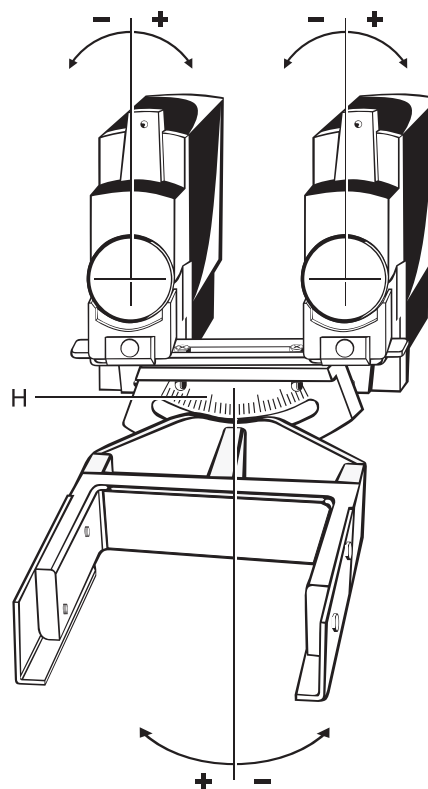
Direction of rotation for angle V for tilting part
