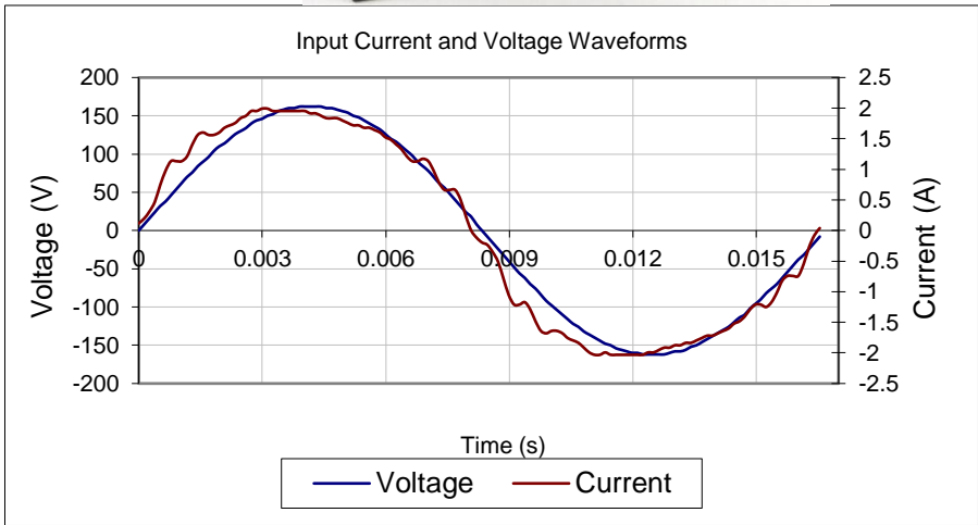
Input AC Current Waveform (ITHD = 11.24%, 50% Load)
