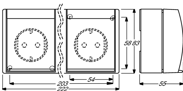
ocean® 3gang horizontal SCHUKO® socket outlets with drilling dimensions
