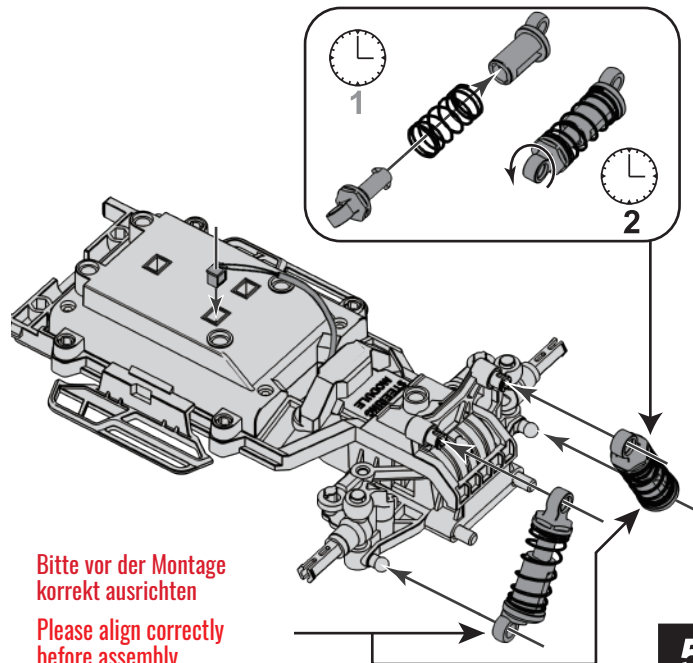
Feder Spring 2x
