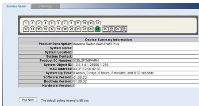
Figure 136 Device View Page
