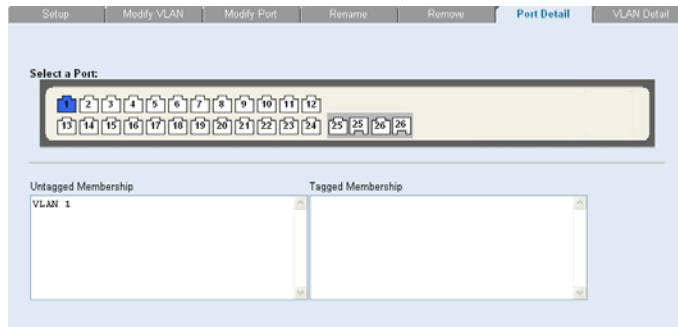
Figure 80 VLAN Port Detail Page
