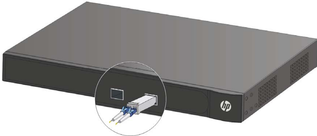
Figure 51 Inserting an SFP Transceiver
