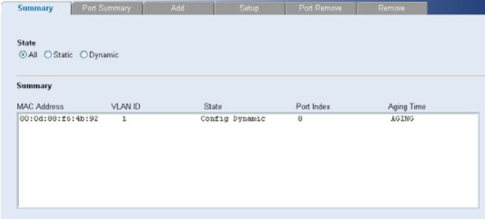
Figure 66 Address Table Summary Page
