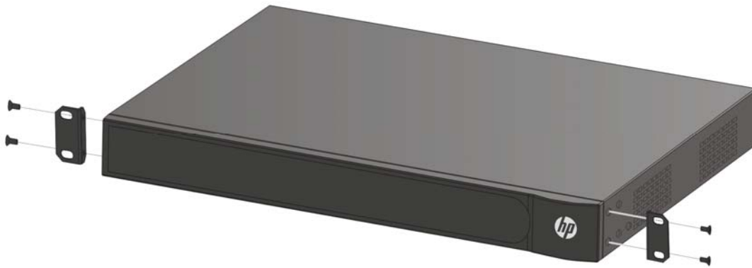
Figure 49 Rack Mounting the Unit
