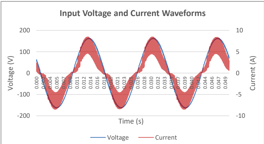
Input AC Current Waveform (ITHD = 15.18%, 50% Load)
