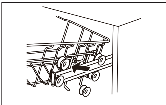
2. Remove the upper basket.
