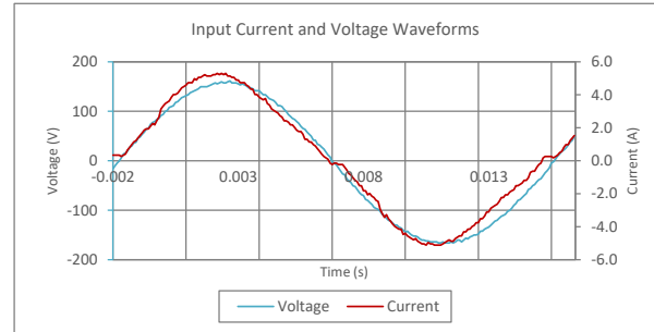
Input AC Current Waveform (I THD = 10.14%, 50% Load)
