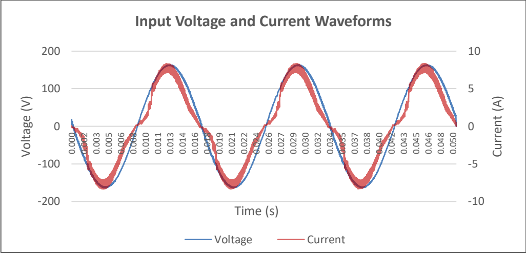
Input AC Current Waveform (ITHD = 17.74%, 50% Load)
