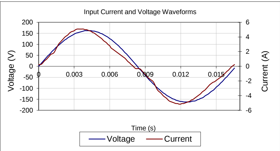
Input AC Current Waveform (ITHD = 11.85%, 50% Load)
